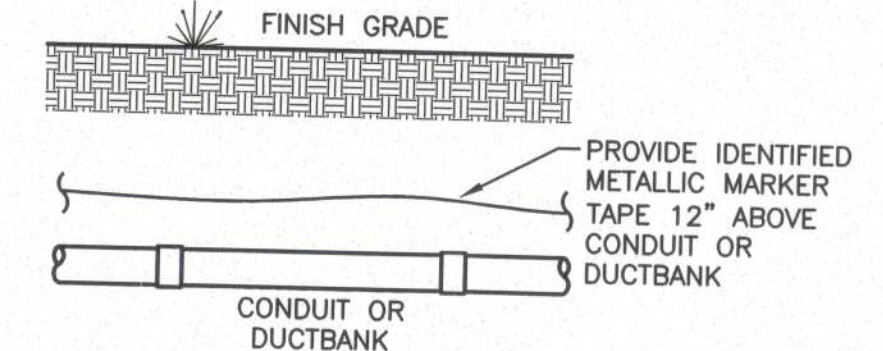
BURIED CONDUIT MARKER DETAIL NOT TO SCALE
