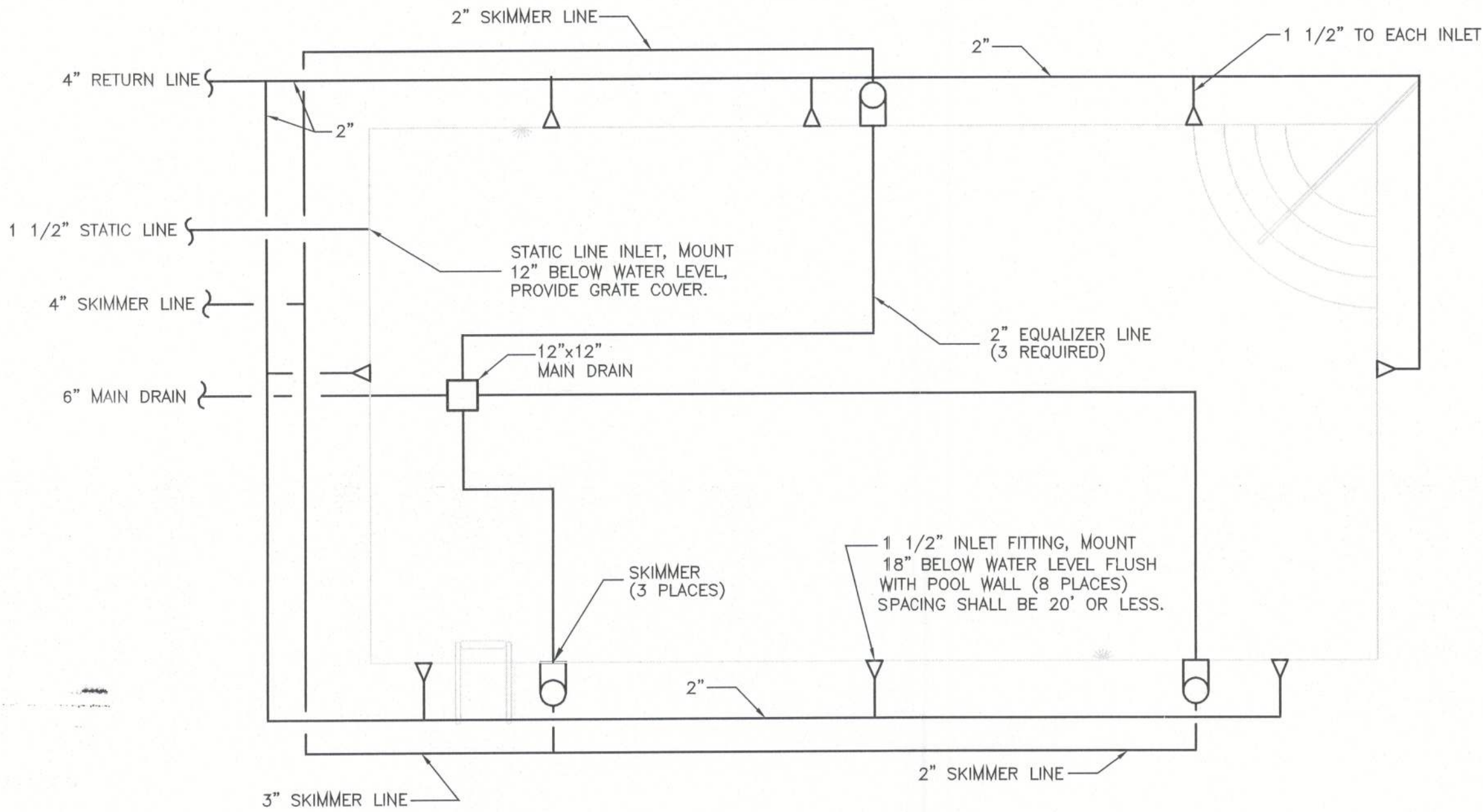
POOL PIPING PLAN SCALE: 1/4"=1'
