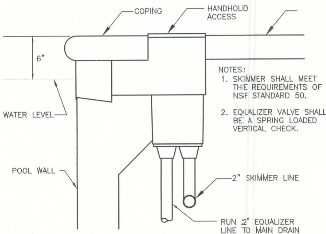
SKIMMER DETAIL SCALE: NONE
