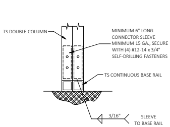
2A RAFTER POST/BASE RAIL CONNECTION DETAIL SCALE: NTS
