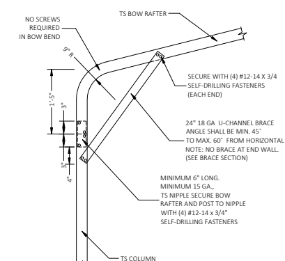
1.2 BOW EAVE RAFTER COLUMN CONNECTION DETAIL FOR HEIGHTS ≤ 12'-0" SCALE: NTS
