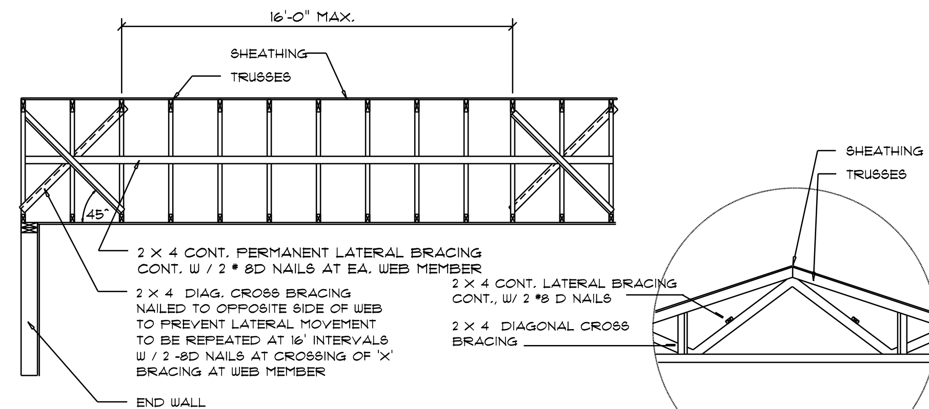
TYP. PERMANENT TRUSS BRACING DIA. NTS NOTE: ALL WOOD TO BE NUMBER 2 GRADE SOUTHERN YELLOW FINE
