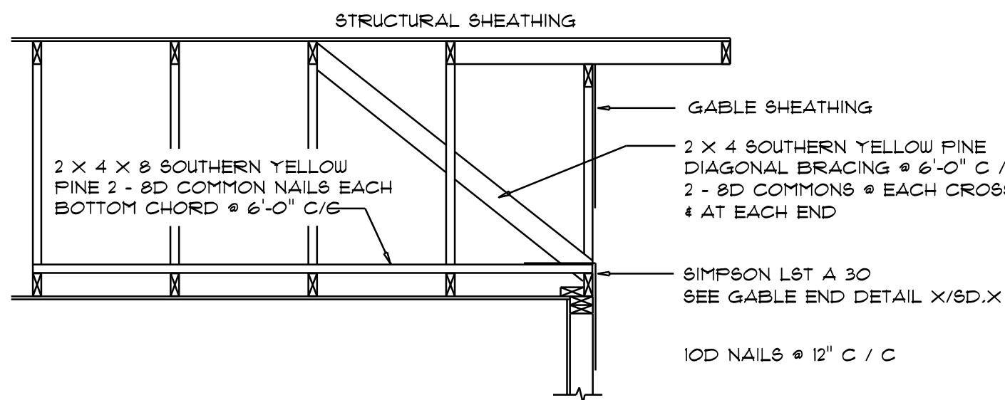
END WALL BRACING FOR CEILING DIAPHRAGM NTS (ALTERNATIVE TO BALLOON FRAMING) NOTE: ALL WOOD TO BE NUMBER 2 GRADE SOUTHERN YELLOW FINE
