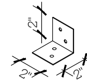
THICKNESS = 14GA ANGLE BRACKET 7 SCALE: NTS
