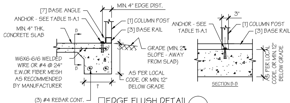
(3) #4 REBAR CONT. EDGE FLUSH DETAIL
