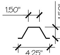
THICKNESS = 14GA / 18GA 4.25" X 1.5" X 18GA / 14GA HAT CHANNEL 5 SCALE: NTS
