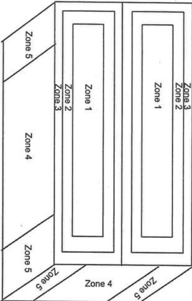
WIND PRESSURE ON COMPONENTS AND CLADDING
