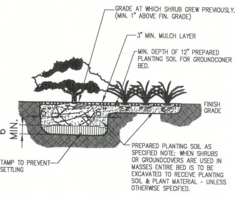
2 SHRUB AND GROUND COVER PLANTING DETAIL NTS
