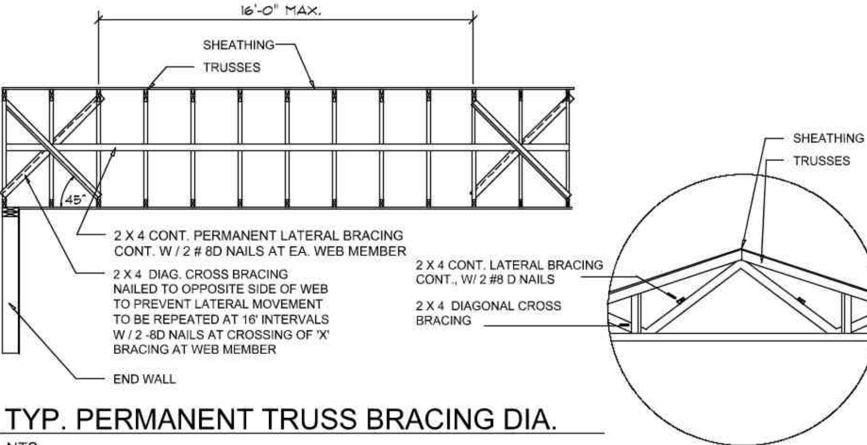
Truss Bracing DETAILS
