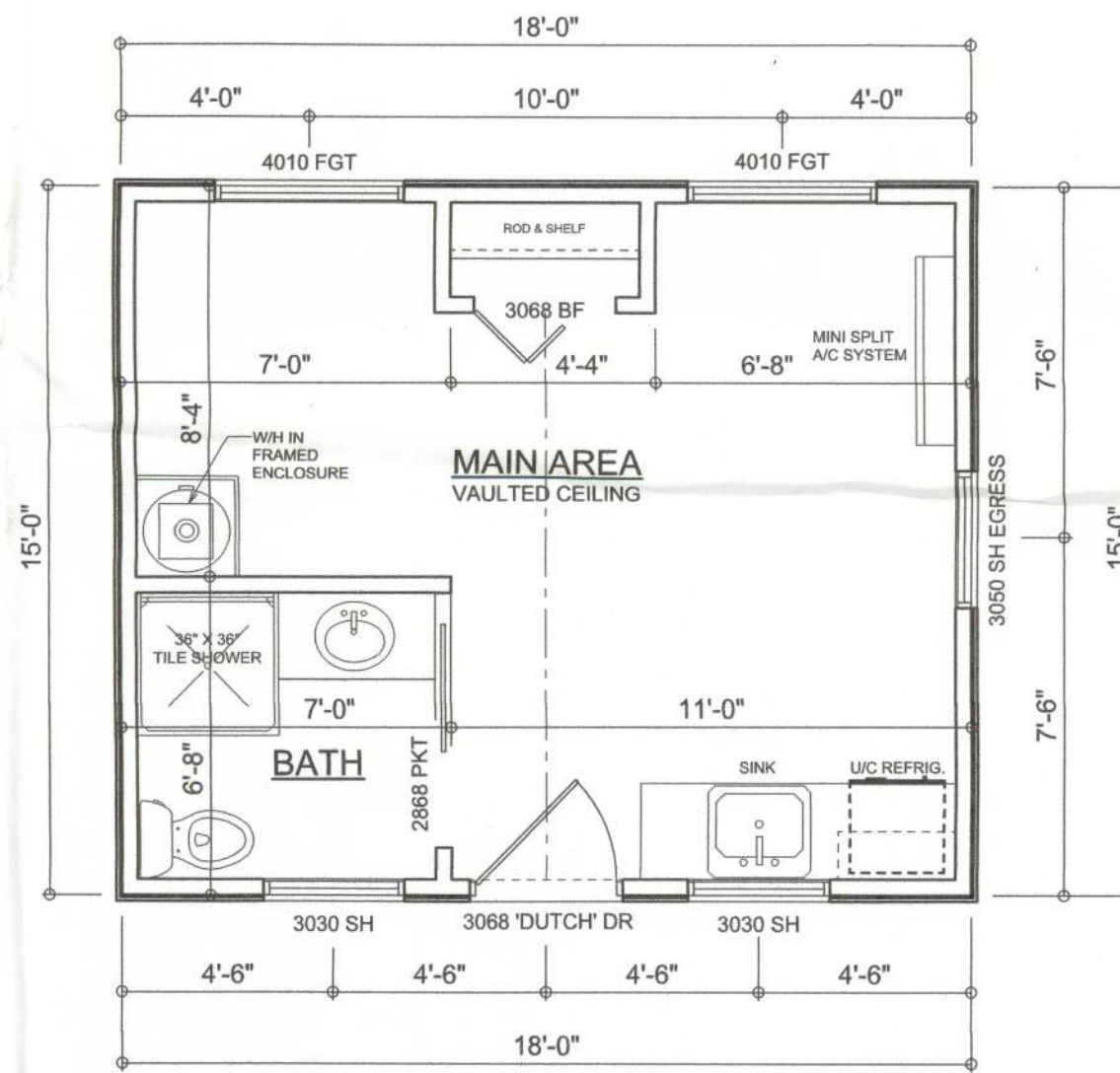
COTTAGE PLAN SCALE: 1/4" = 1'-0" AREA SUMMARY: 270 square feet
