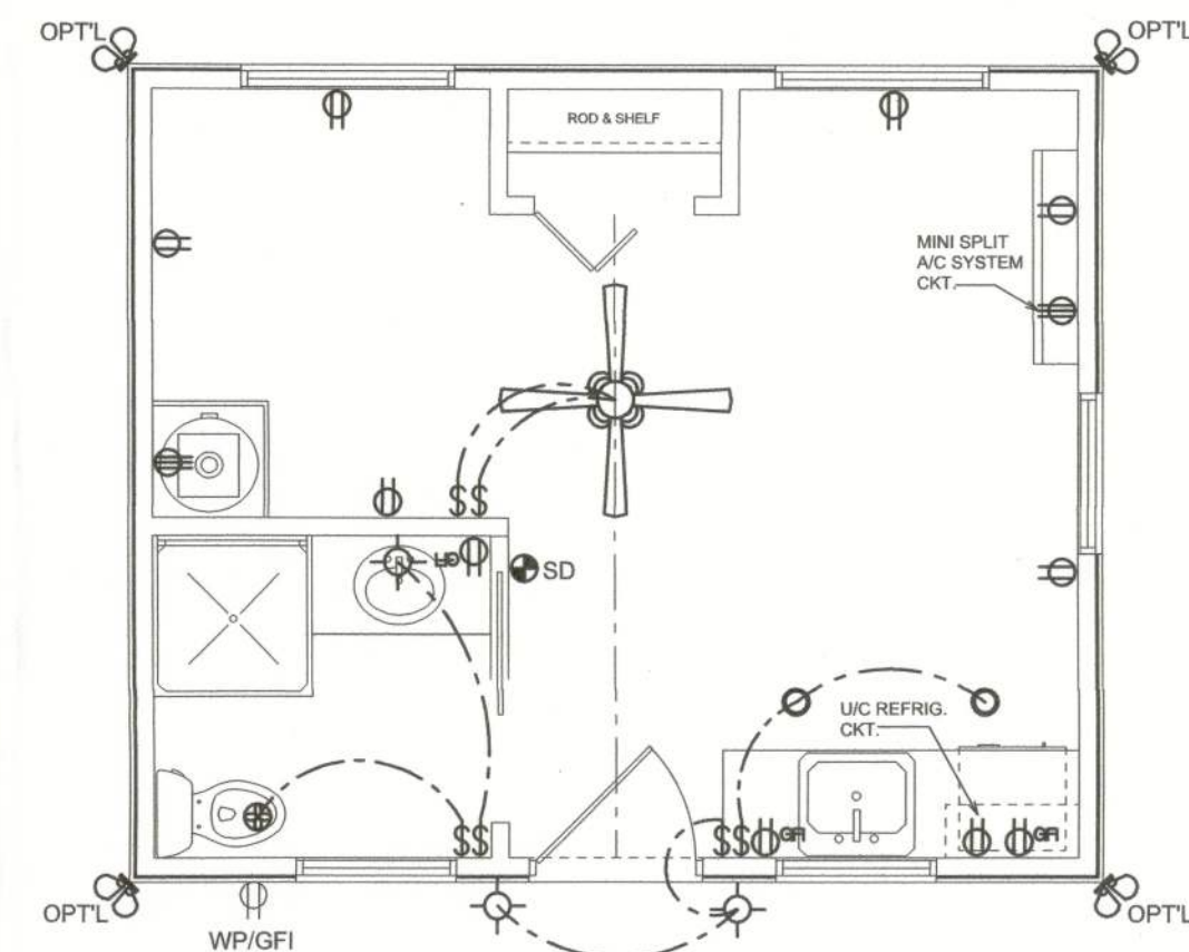
ELECTRICAL PLAN SCALE: 1/4" = 1'-0"
