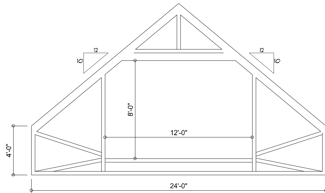
PROPOSED ATTIC TRUSS
