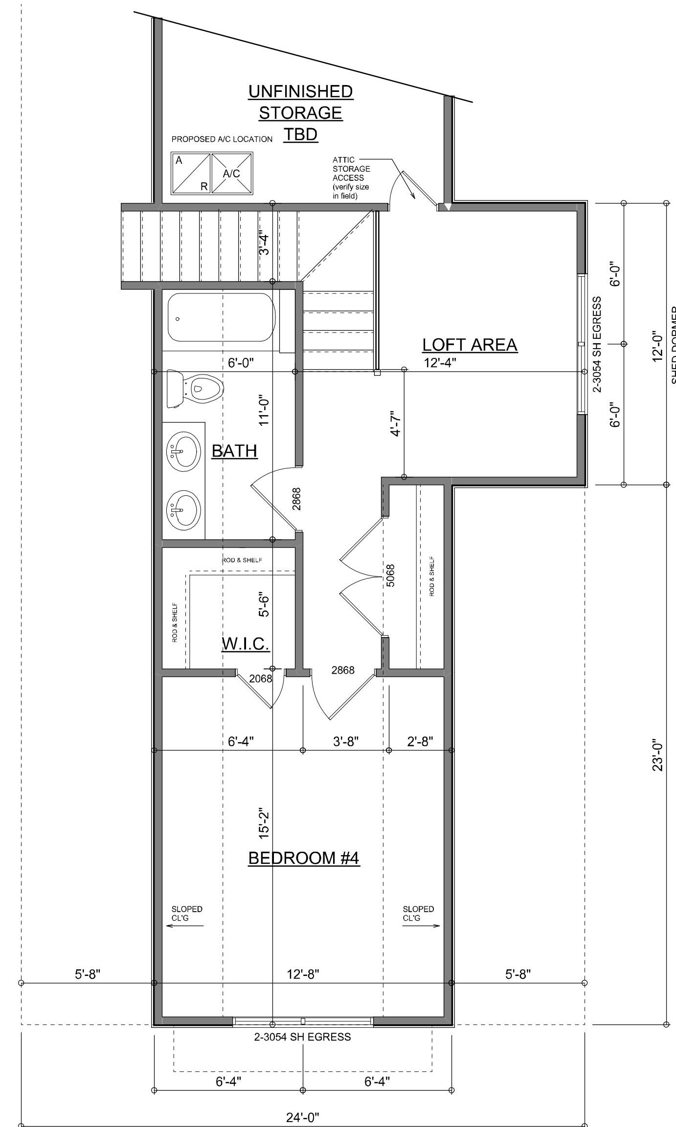
2ND FLOOR PLAN
