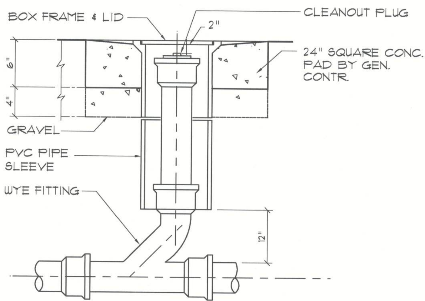
Outdoor Cleanout DETAIL
