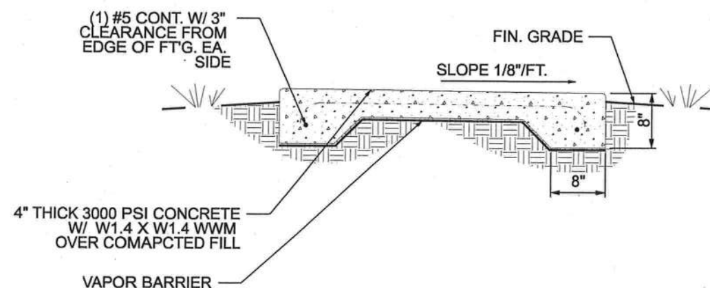
SIDEWALK TYPICAL SECTION NTS
