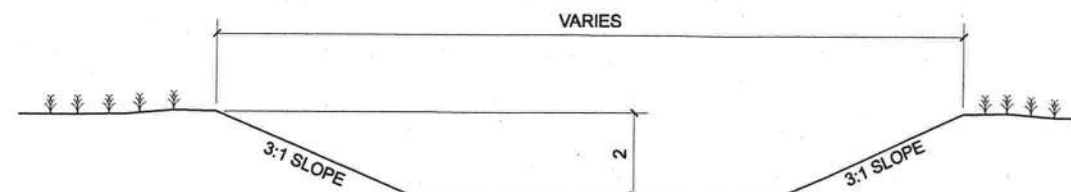
DRAINAGE SWALE DETAIL NTS
