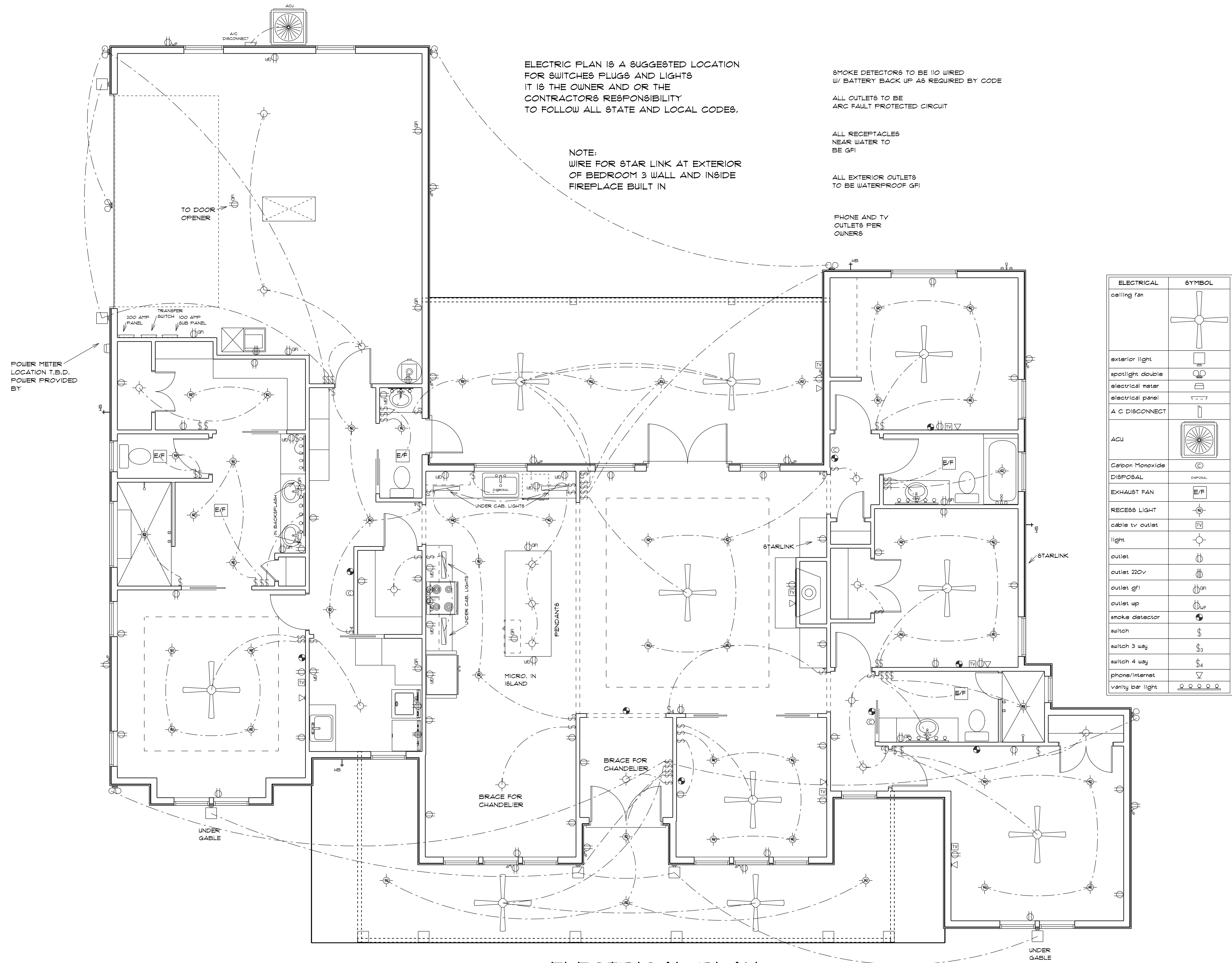
ELECTRICAL PLAN
