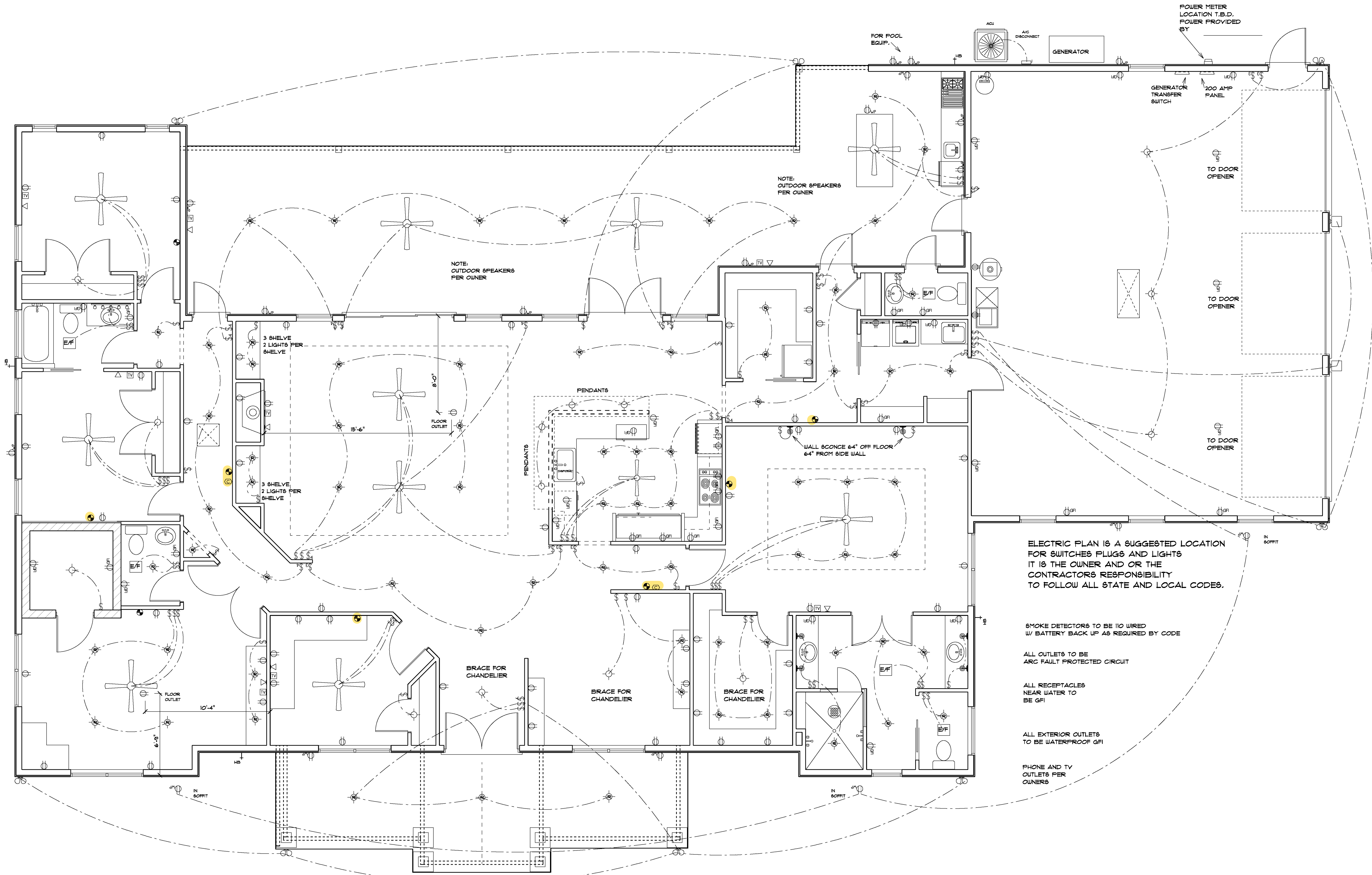
ELECTRICAL PLAN
