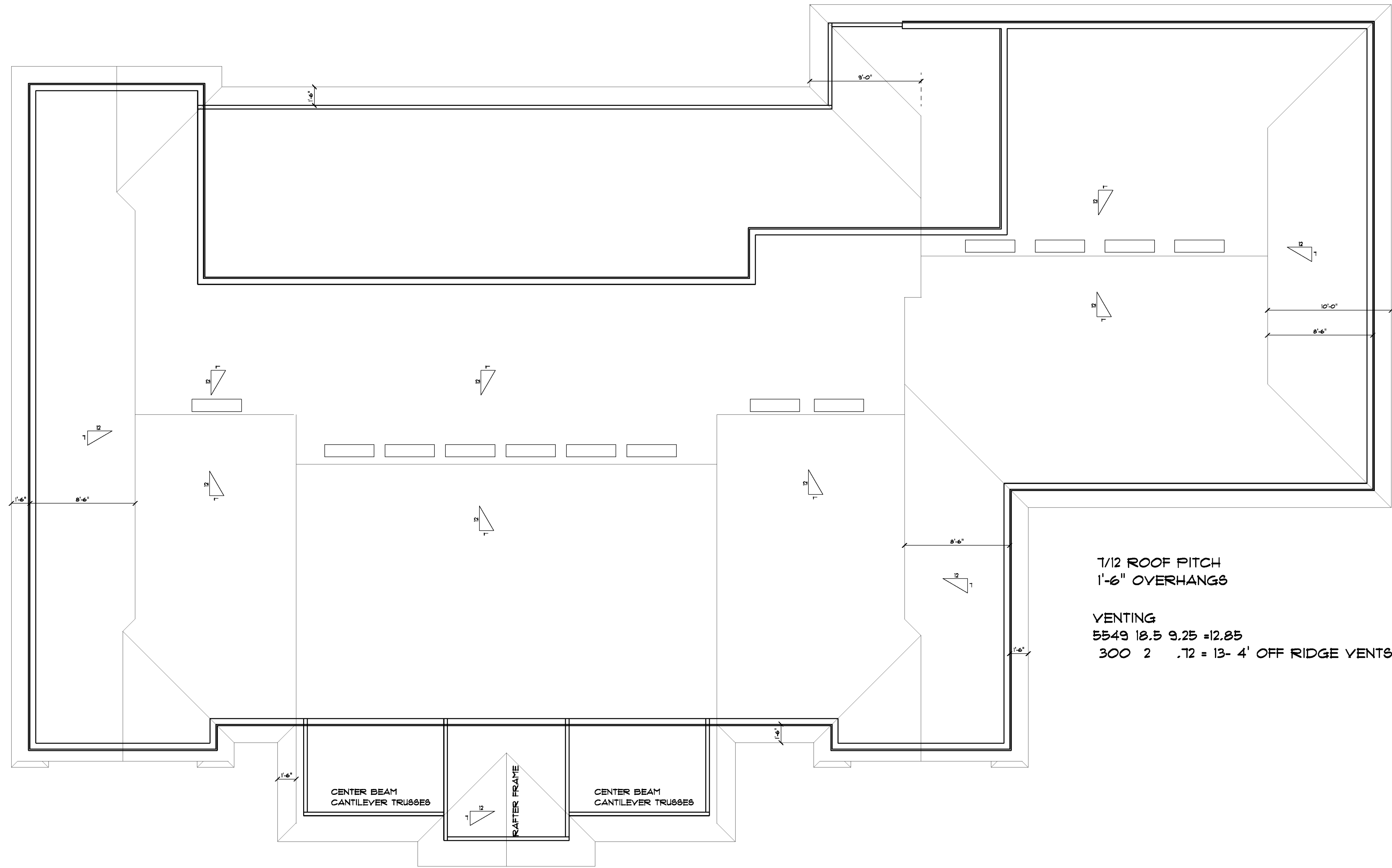
ROOF PLAN 3/16" SCALE
