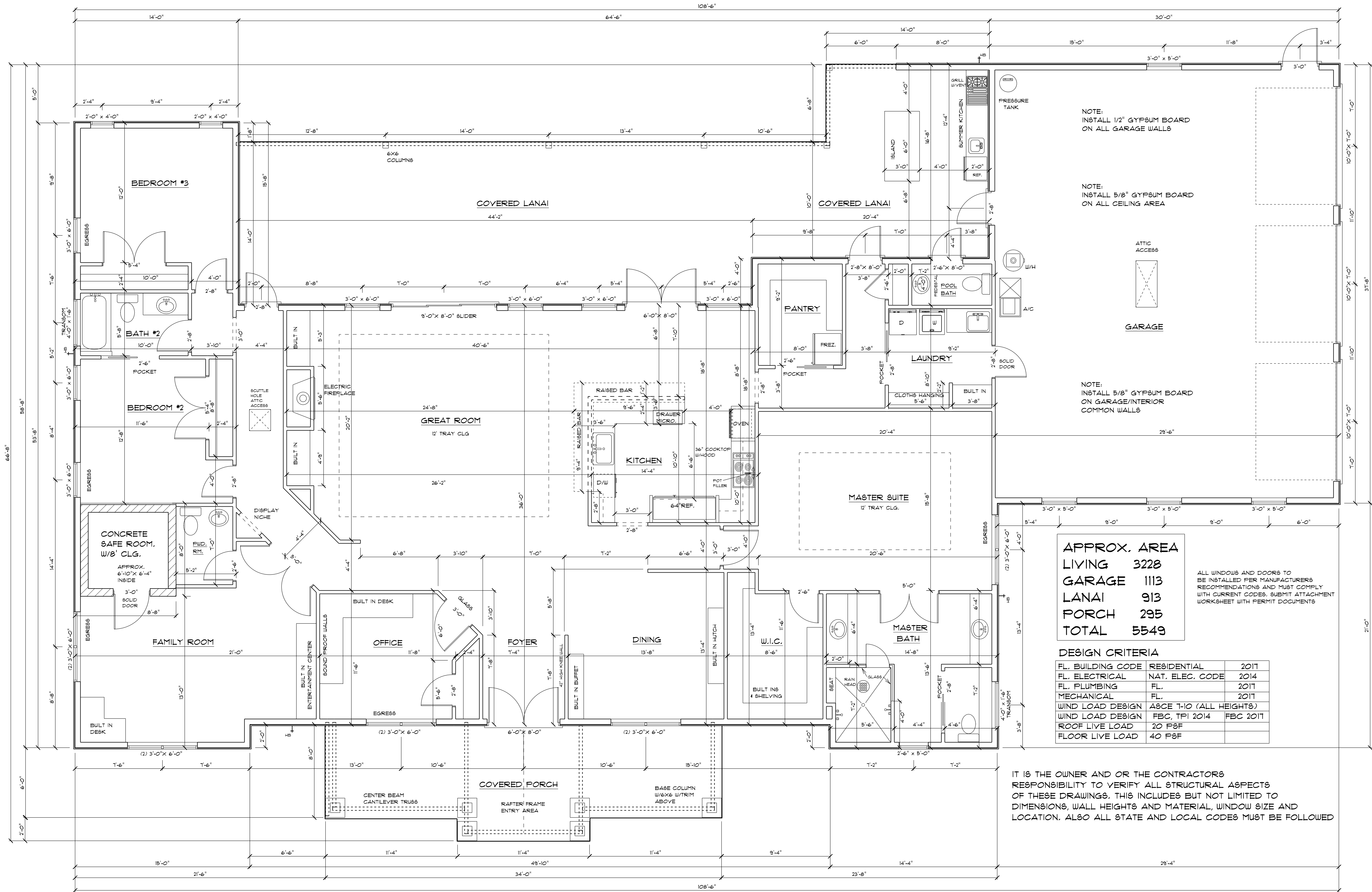
MAIN FLOOR PLAN
