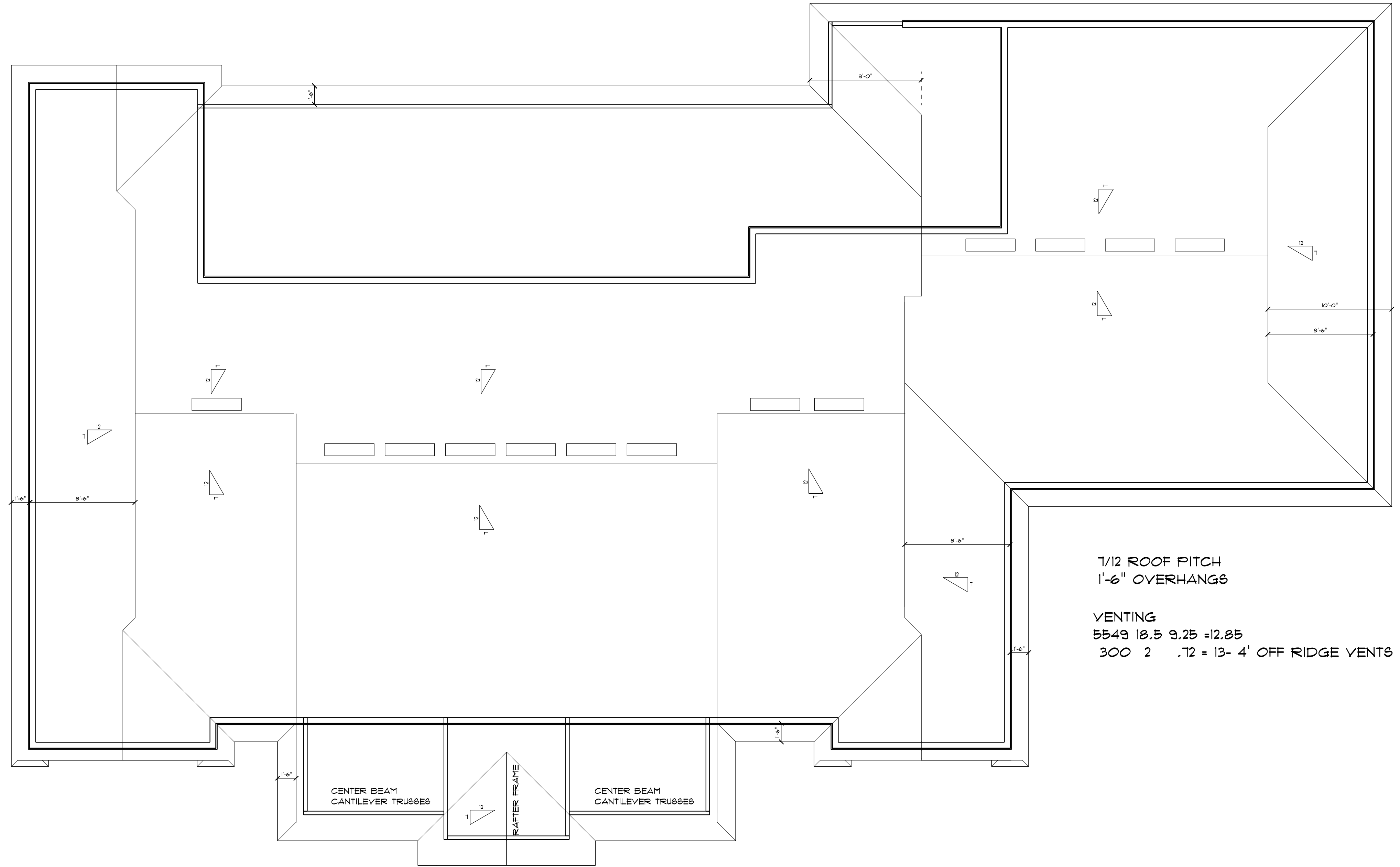
ROOF PLAN
