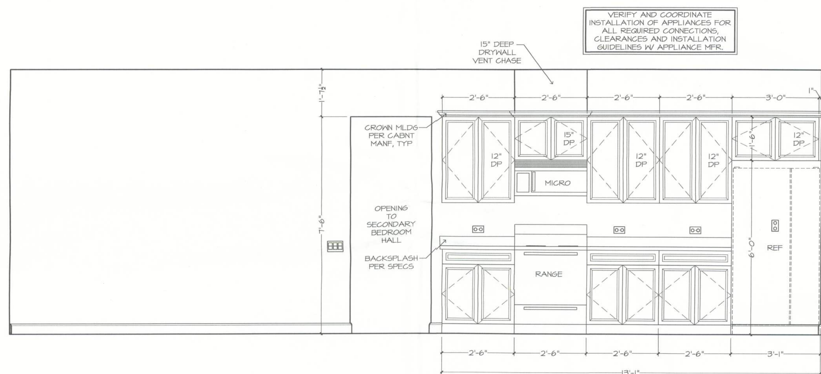
WALL "Y" CASUAL DINING KITCHEN
