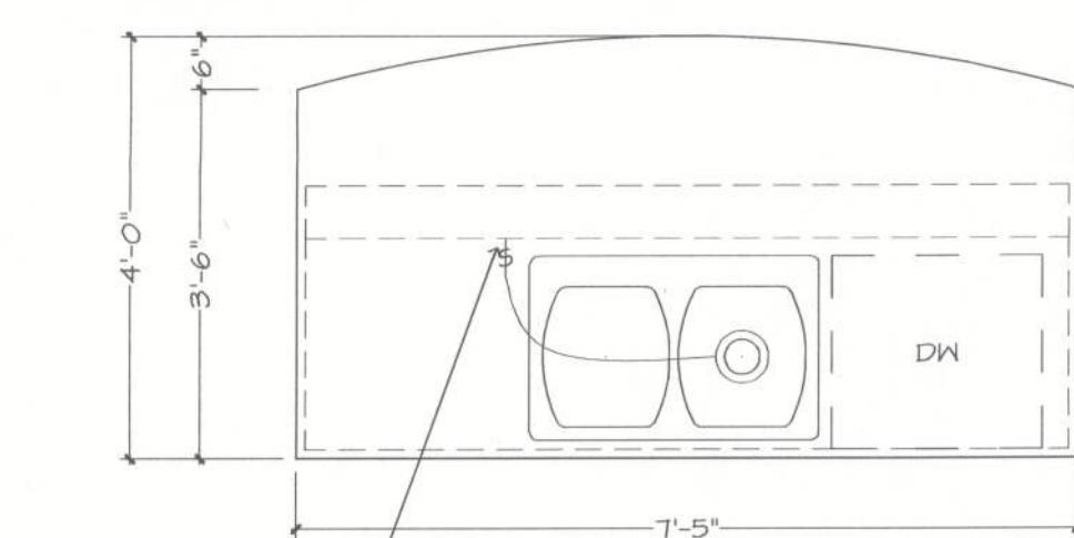
WALL "Y" CASUAL DINING KITCHEN
