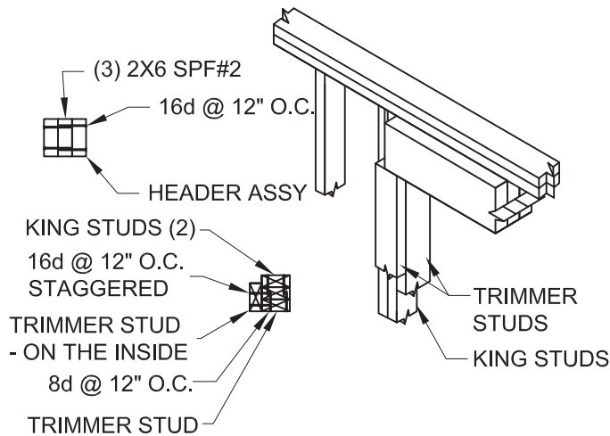
2B TRIPLE HEADER DETAIL FOR SIDE WALLS
