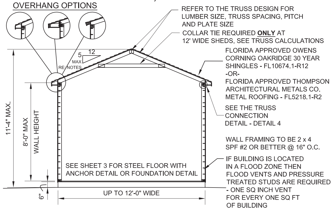
1 BUILDING SECTION
