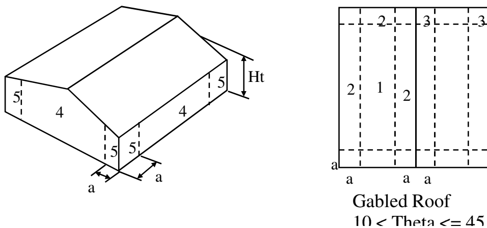
Figure 6-5 - External Pressure Coefficients, GCp
