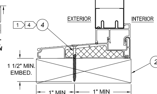
INSWING FIXED UNIT VERTICAL CROSS SECTION
