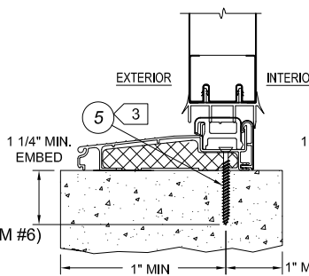
INSWING OPERATING UNIT VERTICAL CROSS SECTION
