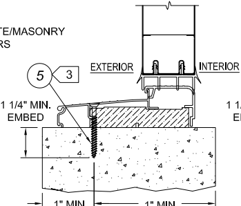
INSWING OPERATING UNIT VERTICAL CROSS SECTION
