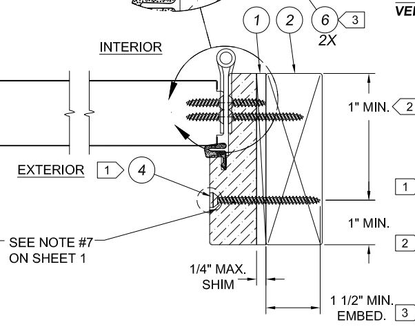
INSWING HINGE JAMB AT FRAME HORIZONTAL CROSS SECTION
