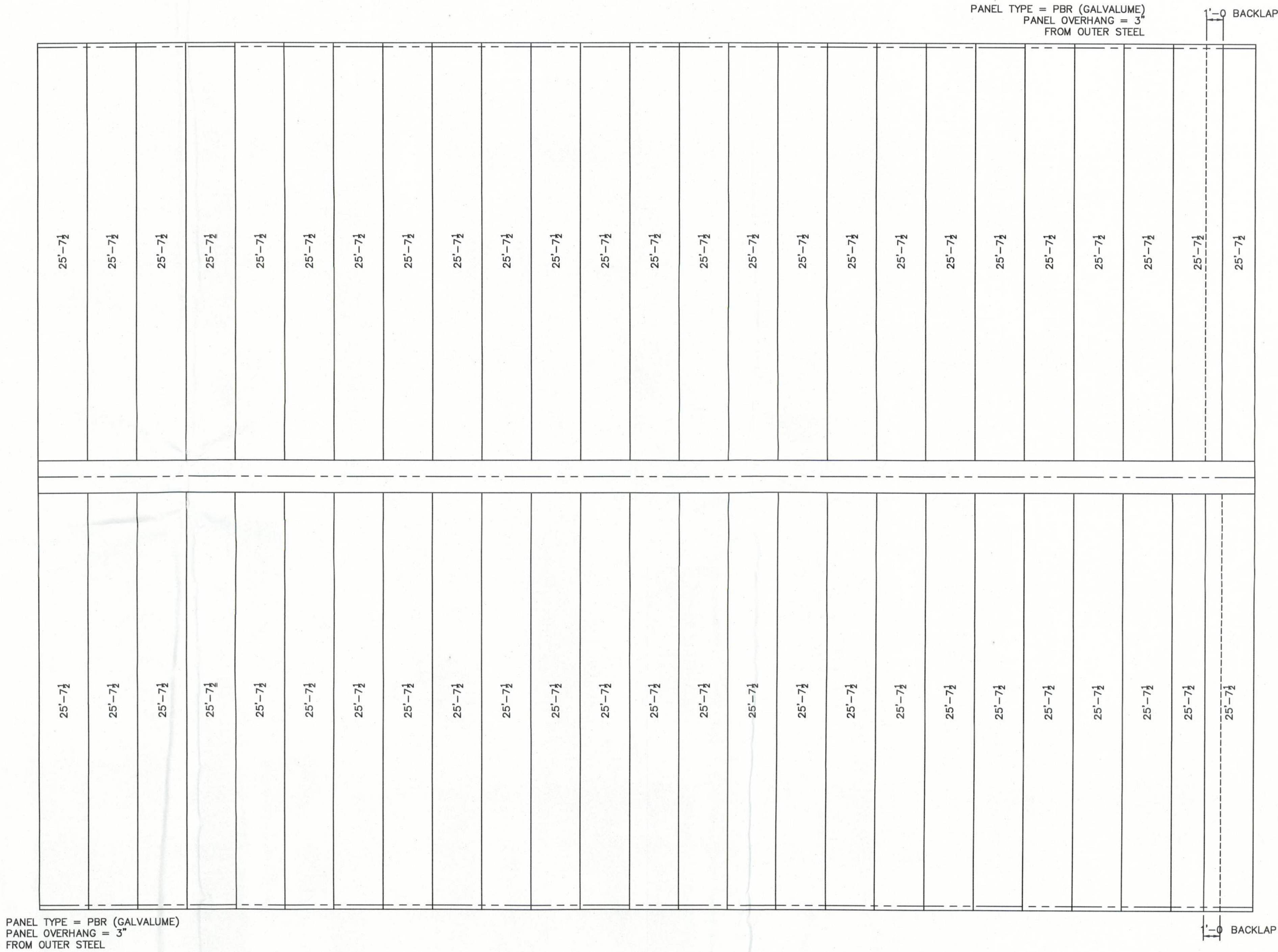
ROOF SHEETING PLAN
