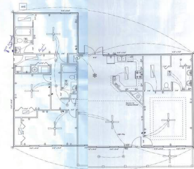
Electrical Plan
