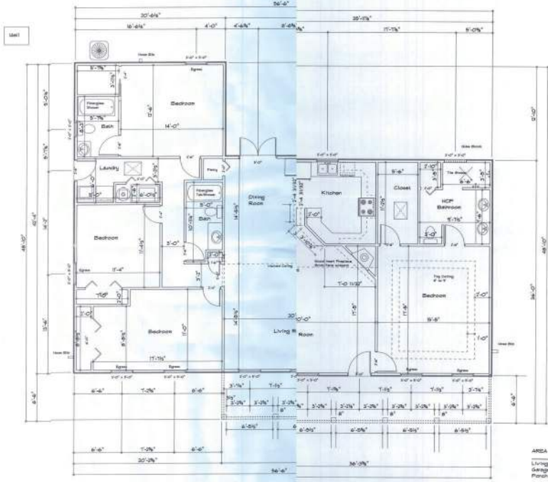
Floor Plan Scale 1/4" = 1'
