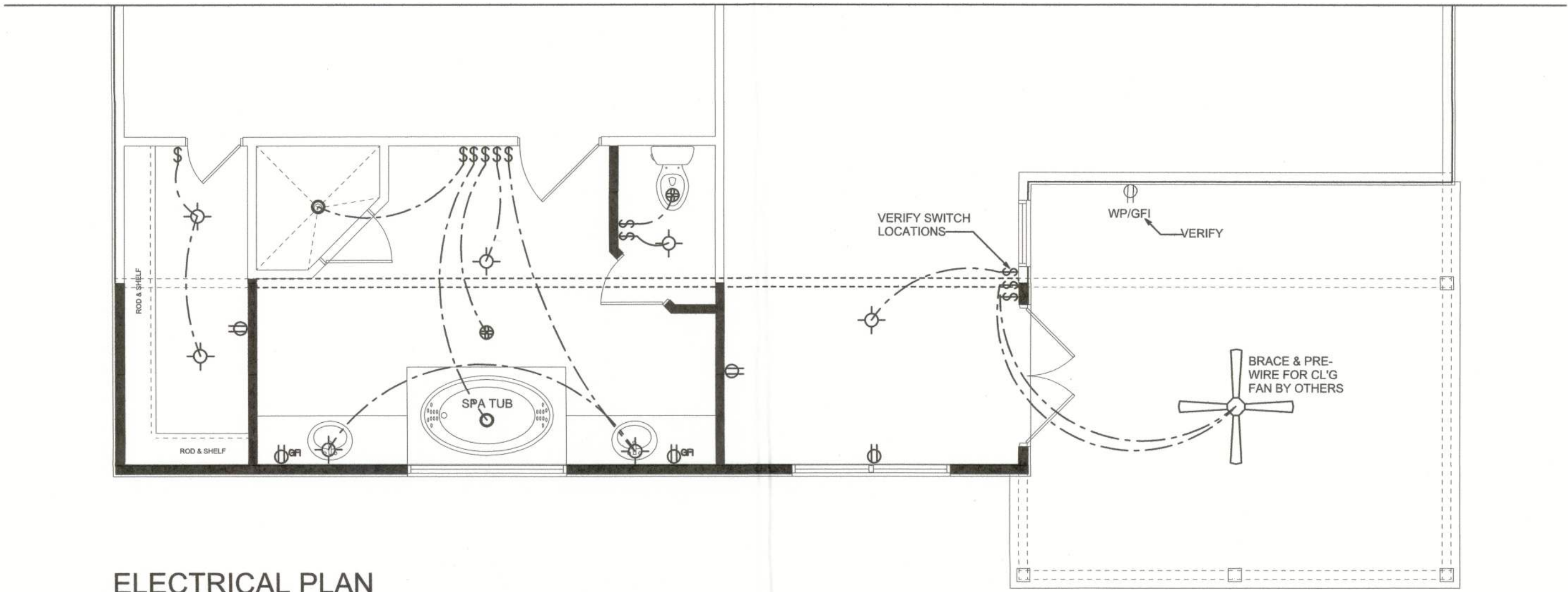
ELECTRICAL PLAN SCALE: 1/4" = 1'-0"
