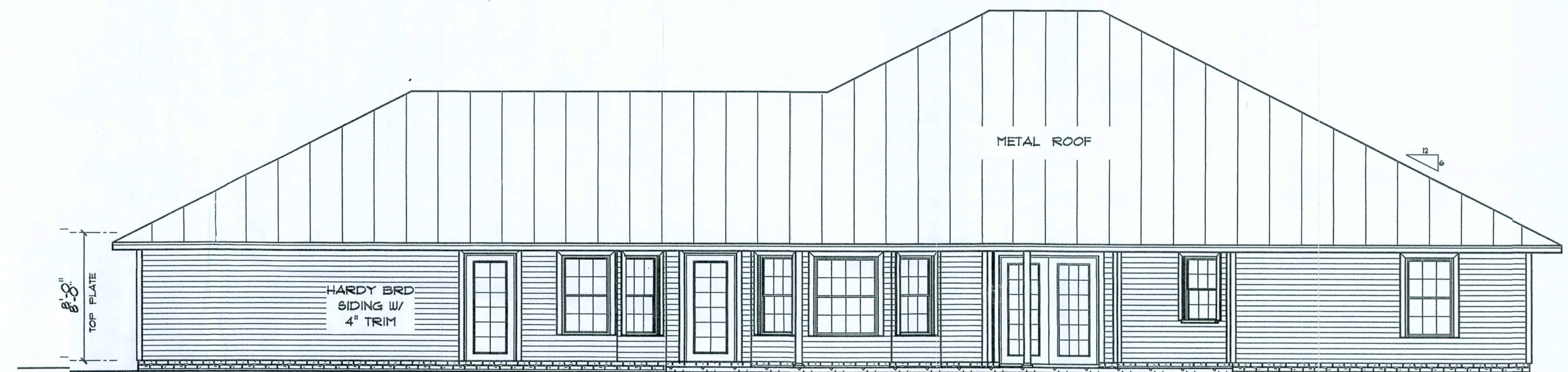
* REAR ELEVATION *
