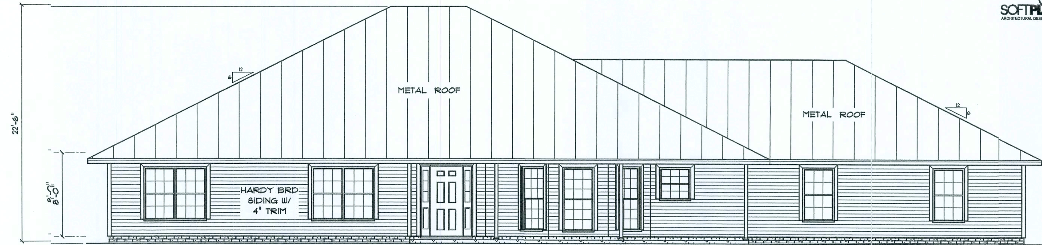
* FRONT ELEVATION *
