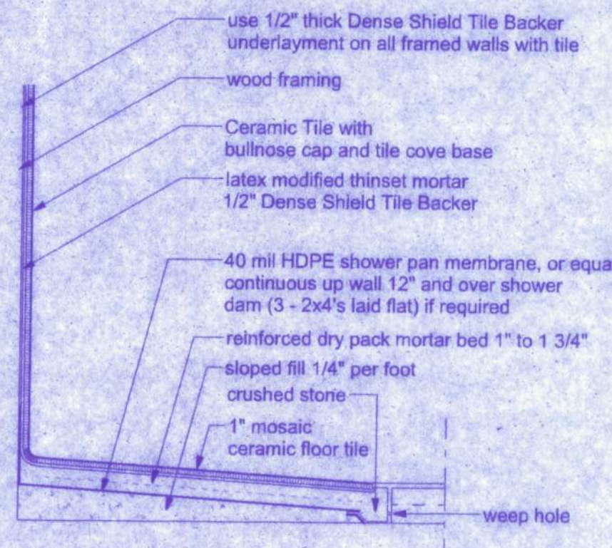
TILE SHOWER
