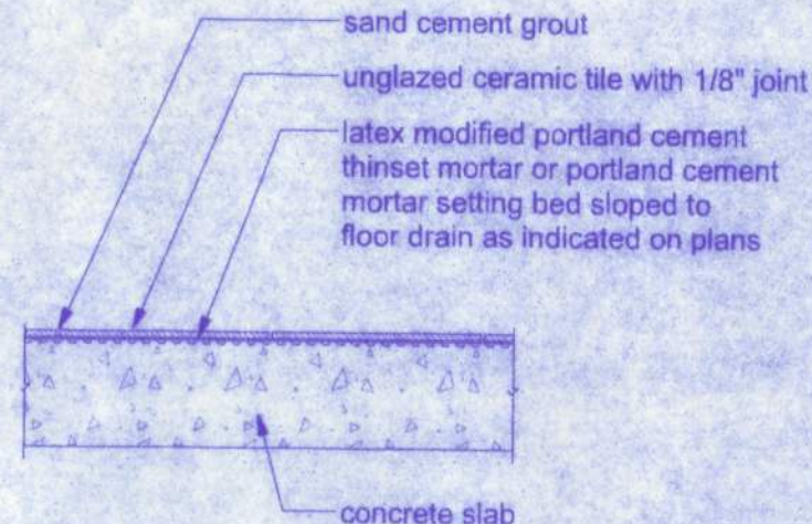
CERAMIC TILE FINISH
