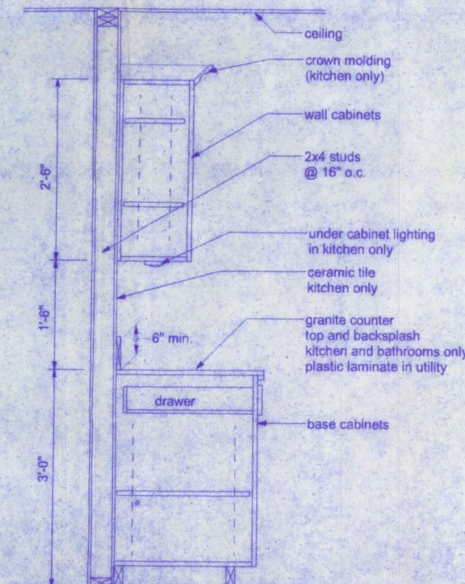
A CABINET SECTION SCALE: 3/4" = 1'-0"
