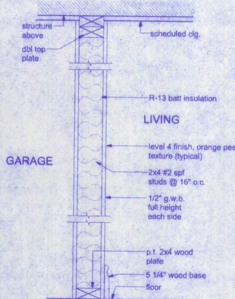
1 GARAGE PARTITION
