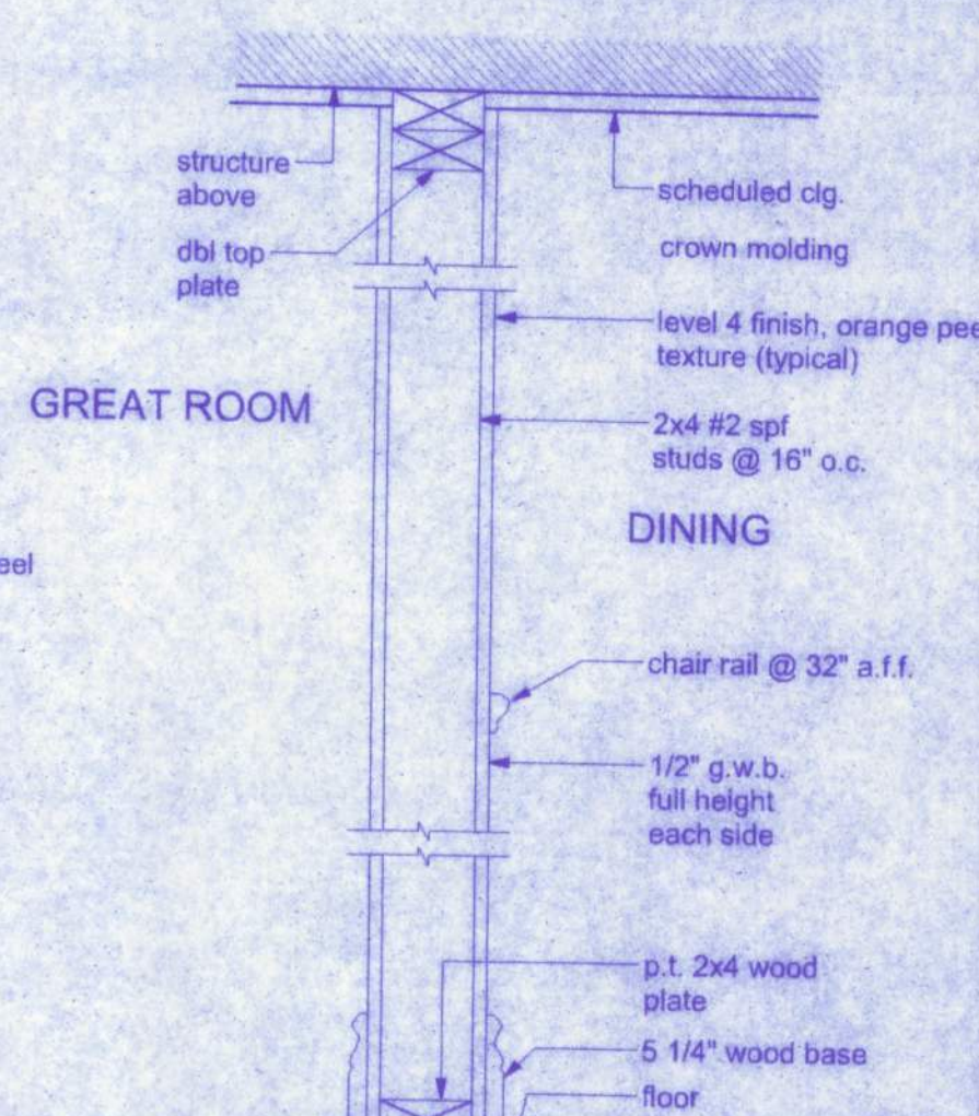
FULL HEIGHT PARTITION
