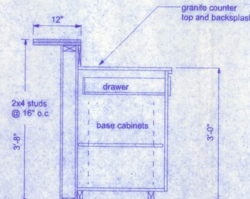
B CABINET SECTION SCALE: 3/4" = 1'-0"
