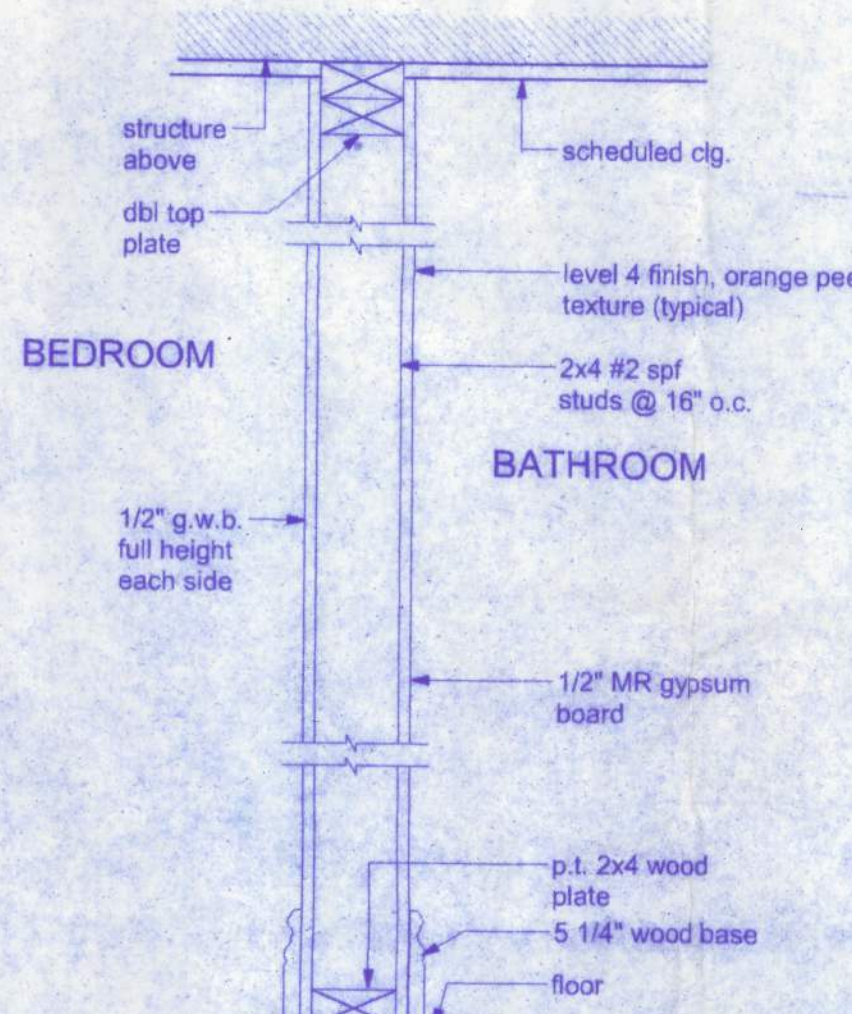
4 FULL HEIGHT PARTITION
