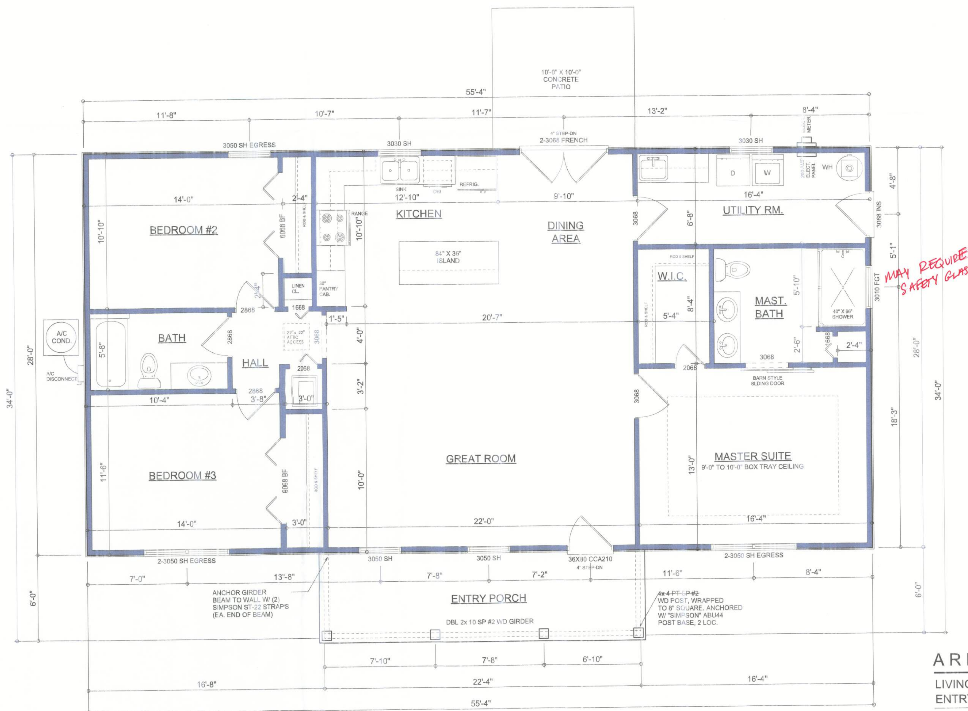
DIMENSIONED FLOOR PLAN SCALE: 1/4" = 1'-0" NOTE: ALL WALLS SHALL BE 9'-0" UNLESS OTHERWISE NOTED.
