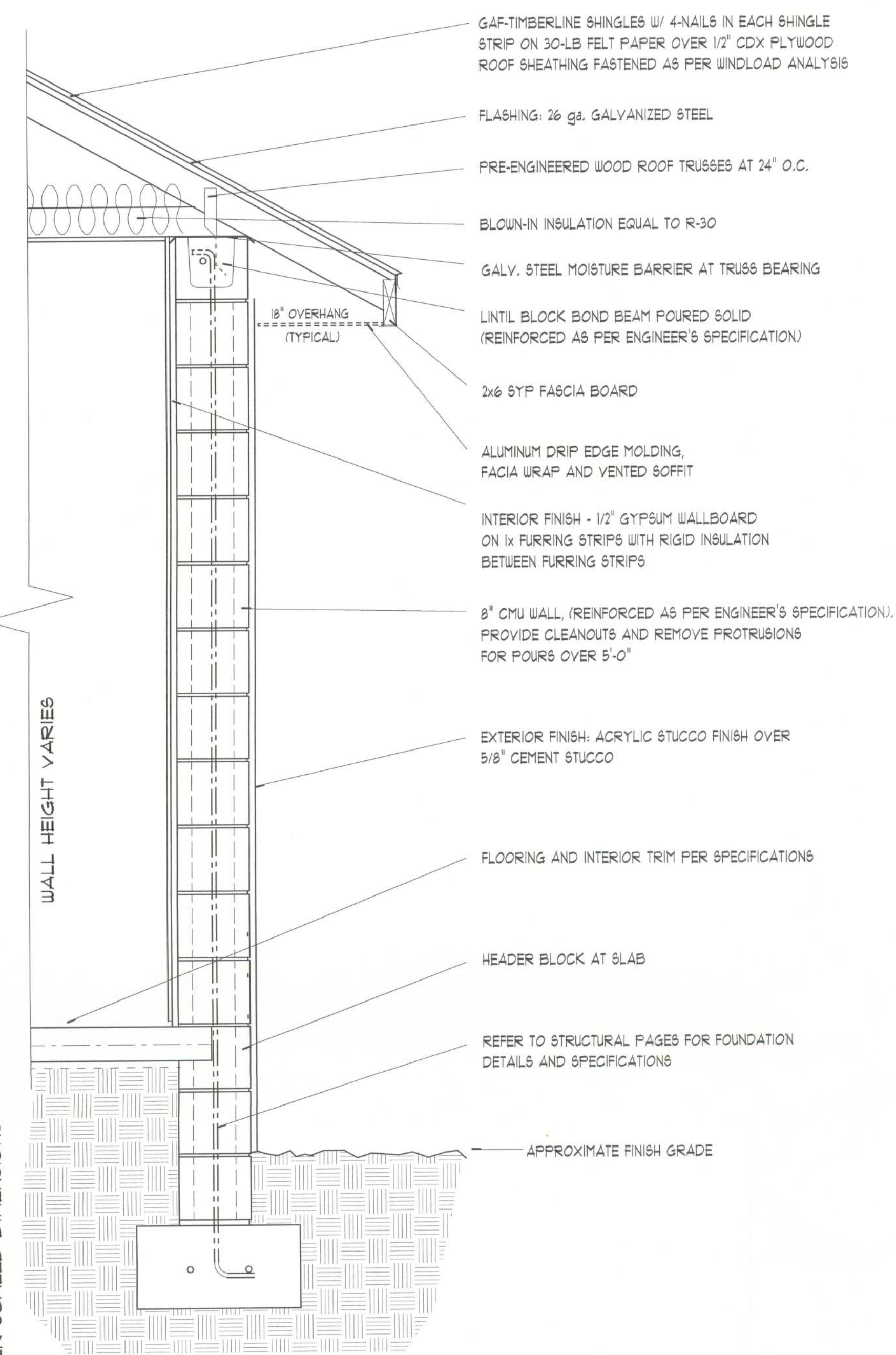
TYPICAL WALL SECTION SCALE: 1" = 1'
