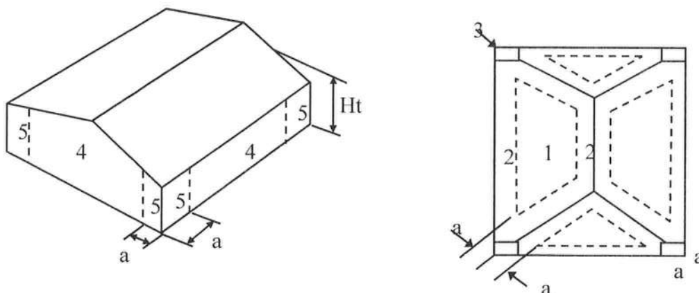
Figure 6-5 - External Pressure Coefficients, GCp Loads on Components and Cladding for Buildings w/ Ht ≤ 60 ft
