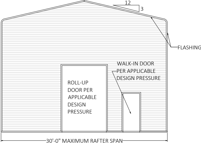
TYPICAL END ELEVATION - BOW EAVE
