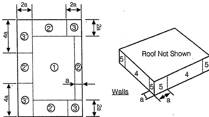
Wind Pressure Summary for C&C Zones based Upon Areas Ch 30 Pt 1 (Table 1 of 2) All wind pressures include a load factor of 0.6
