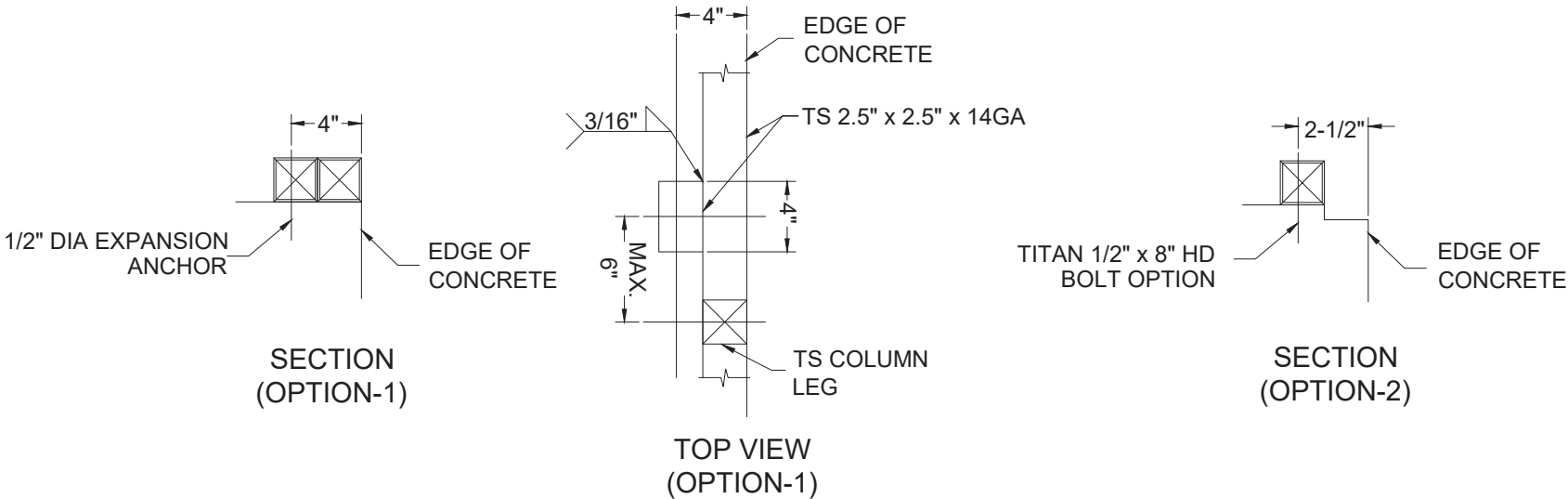
3D TYPICAL ANCHOR DETAIL WHEN BASE RAIL IS NEAR EDGE OF CONCRETE SCALE: NTS
