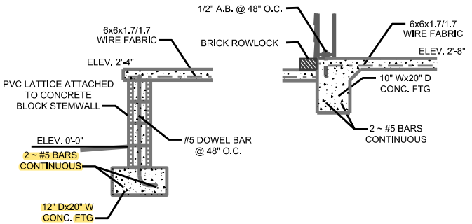
FOUNDATION DETAIL 1 NOTE: FAUX BRICK COLUMN PIERS NOT SHOWN
