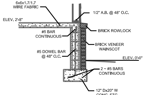
FOUNDATION DETAIL 2
