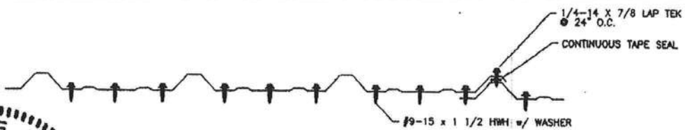
FASTENER PATTERN AT EAVE & VALLEY
