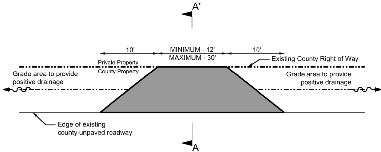
Driveway Connection Plan View
