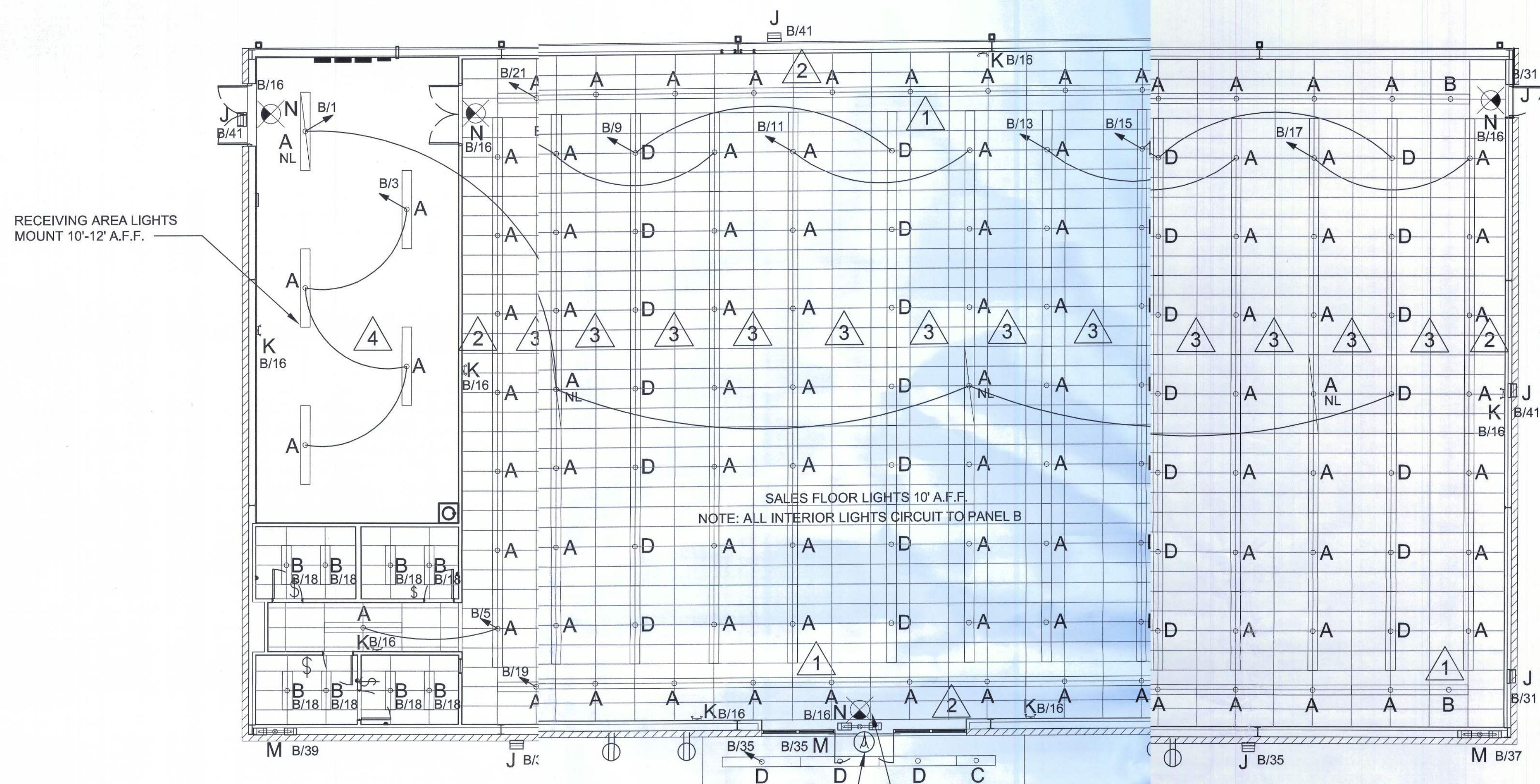
1 LIGHTING PLAN E2.C 1/16" = 1'-0"
