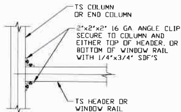
COLUMN OR WINDOW RAIL/ WALL GIRT TO POST CONNECTION DETAIL SCALE: NTS
