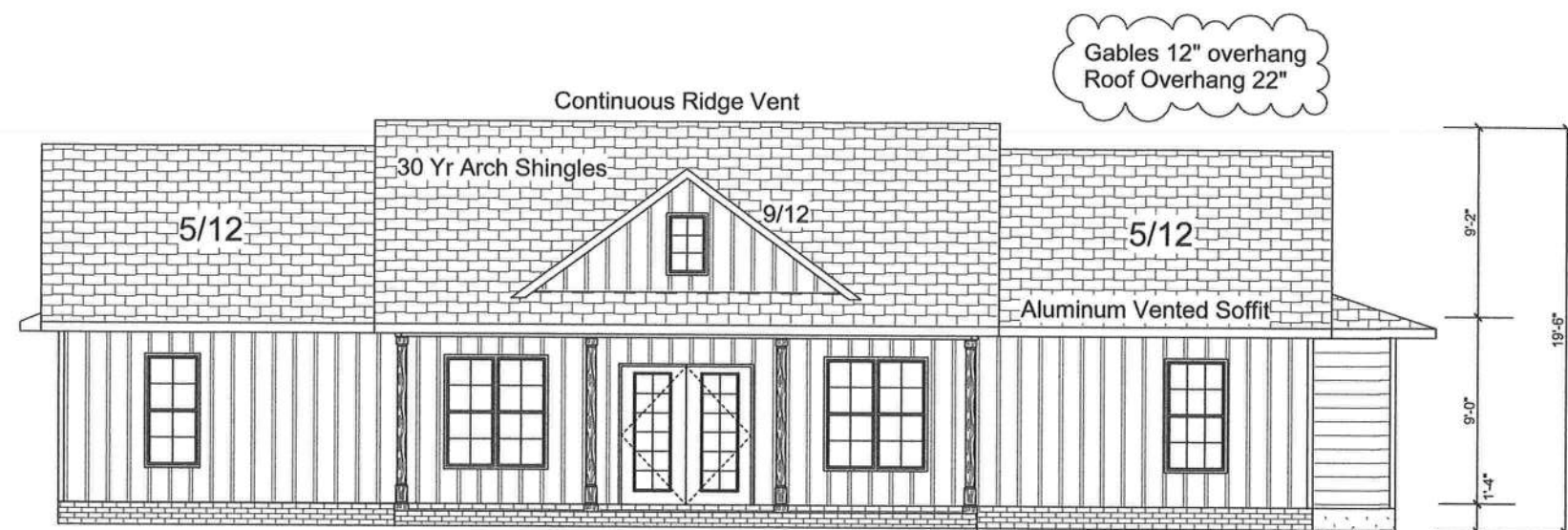
Front Elevation opt 1
