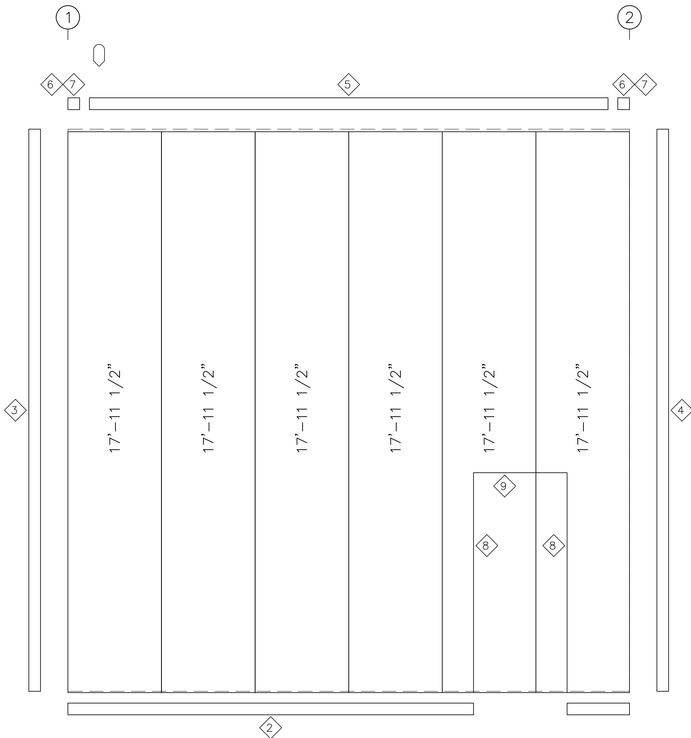
SIDEWALL SHEETING & TRIM: FRAME LINE I
