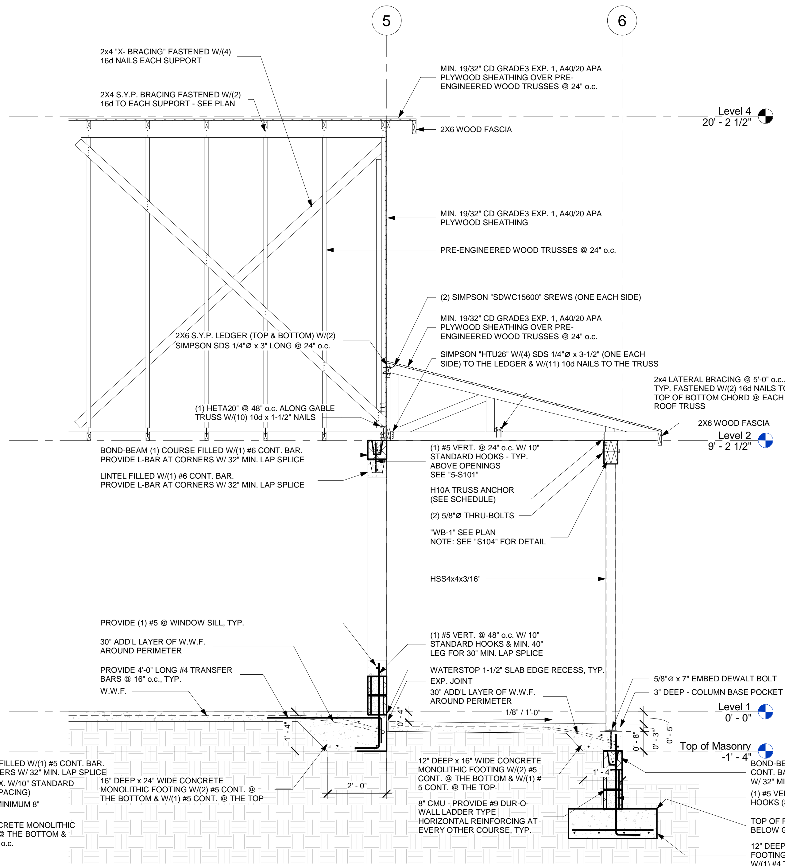
1 Structural Building Section 1 1/2" = 1'-0"
