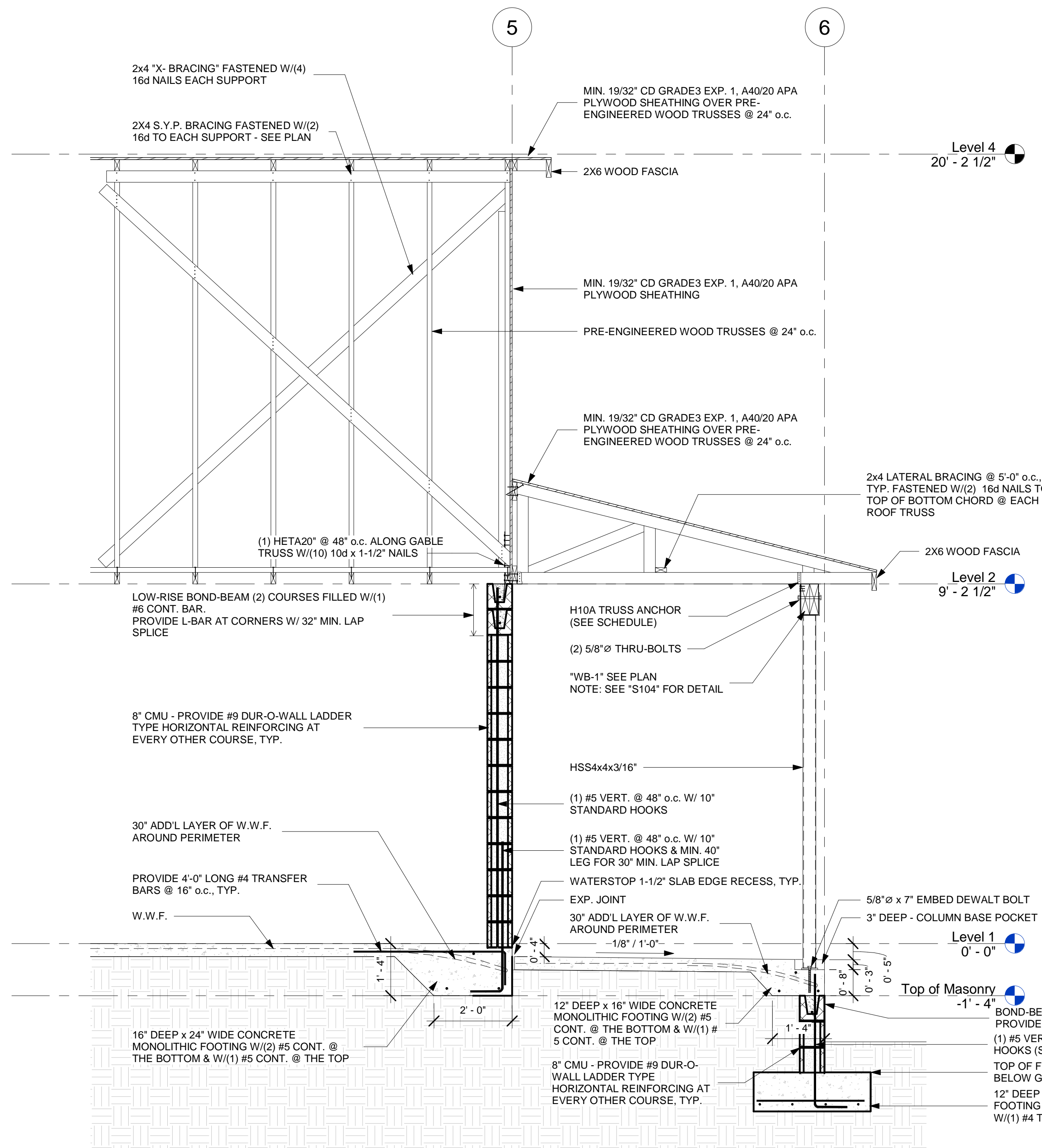
2 Structural Building Section 2 1/2" = 1'-0"
