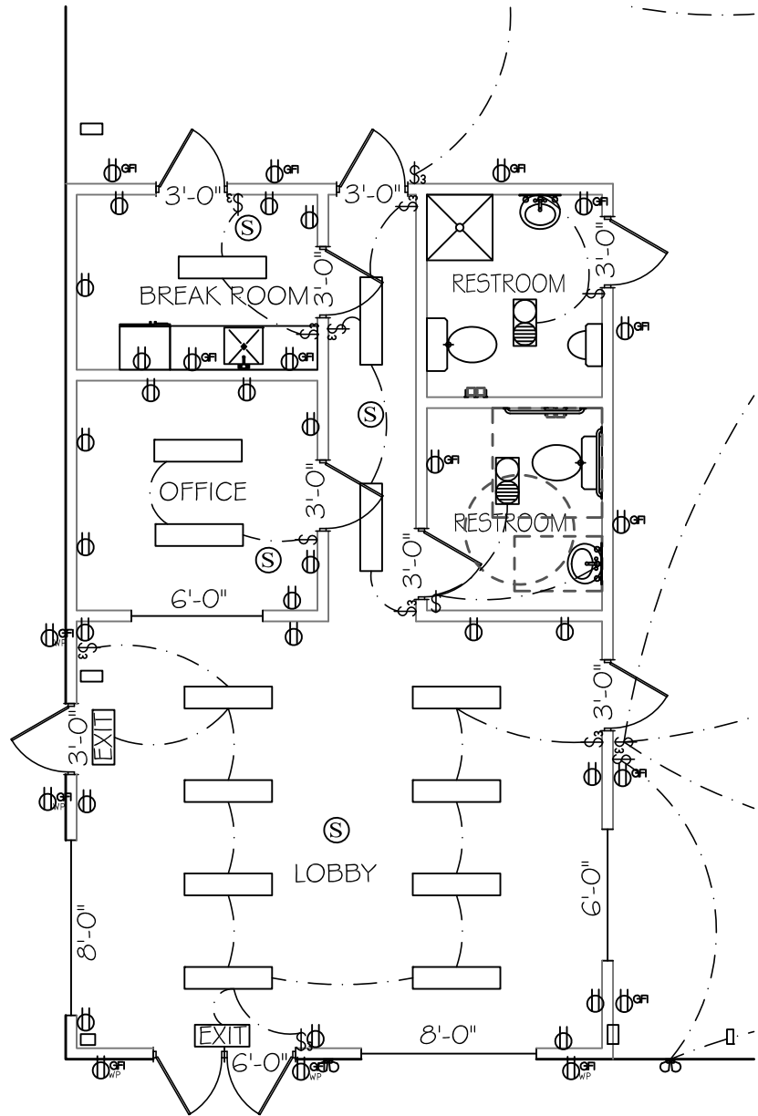
ELECTRICAL PLAN
