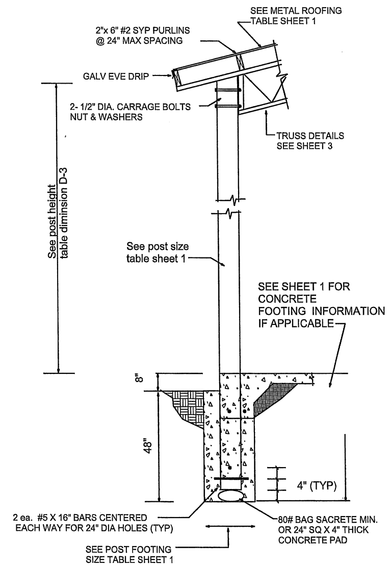
POST FOOTING TO TRUSS DETAIL 1
