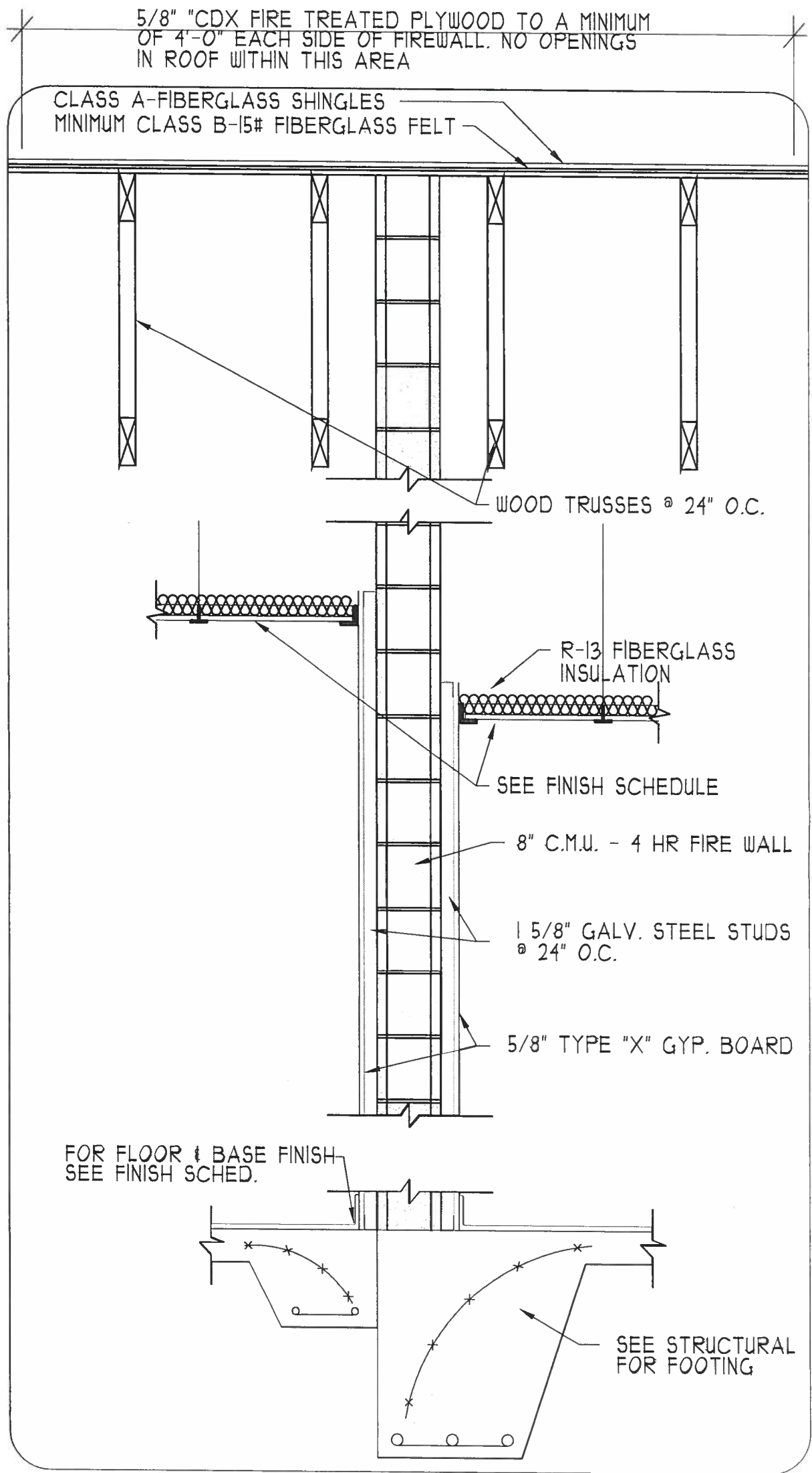
M SECTION @ 4-HOUR FIRE WALL A5.1 3/4" = 1'-0"
