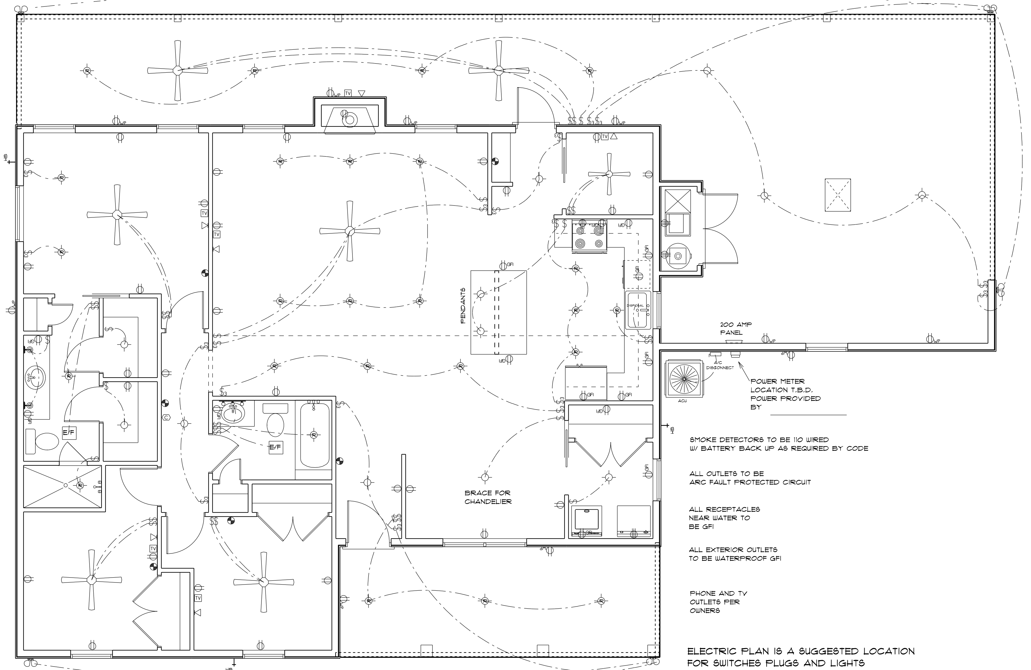
ELECTRICAL PLAN
