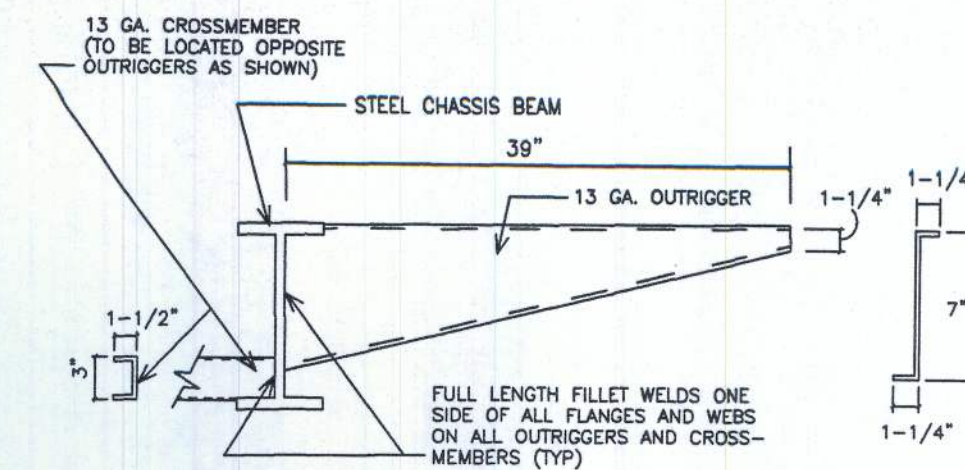
OUTRIGGER AND CROSSMEMBER SECTIONS
