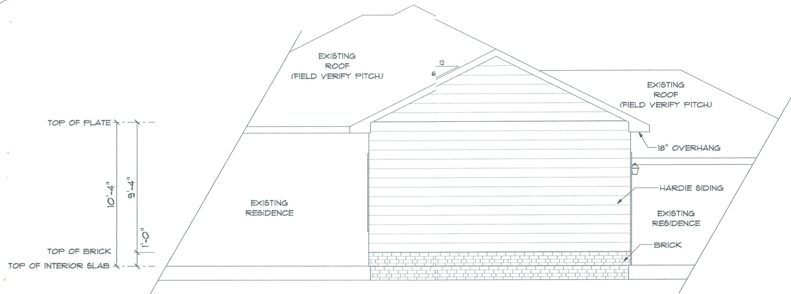
FRONT ELEVATION
