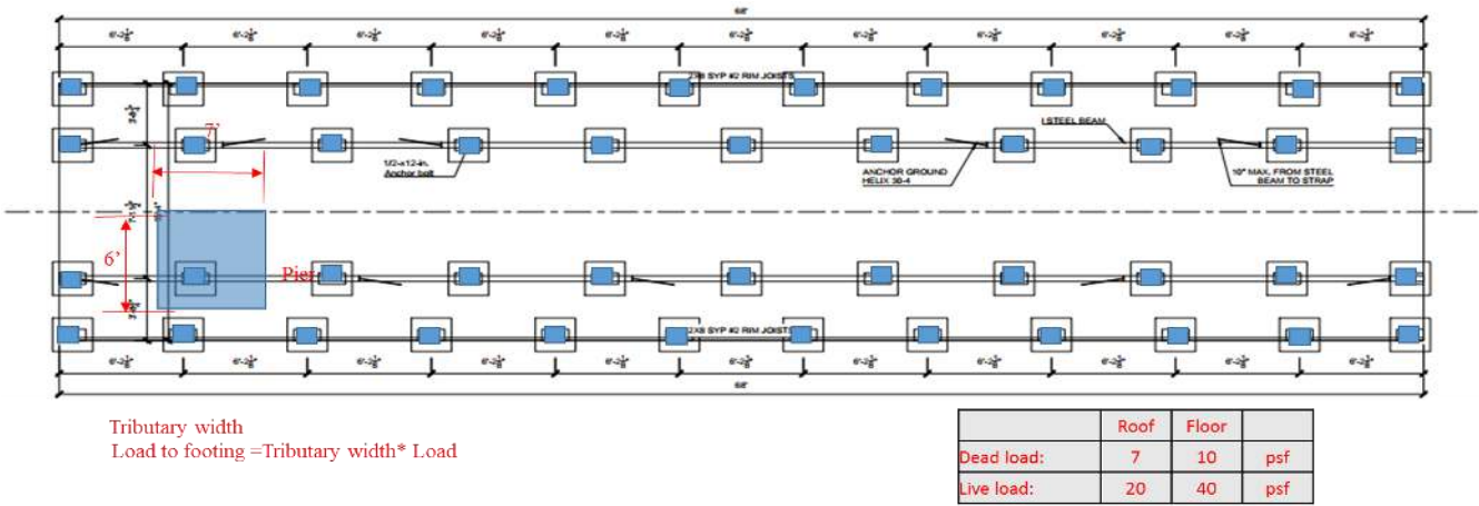
Foundation Plan
