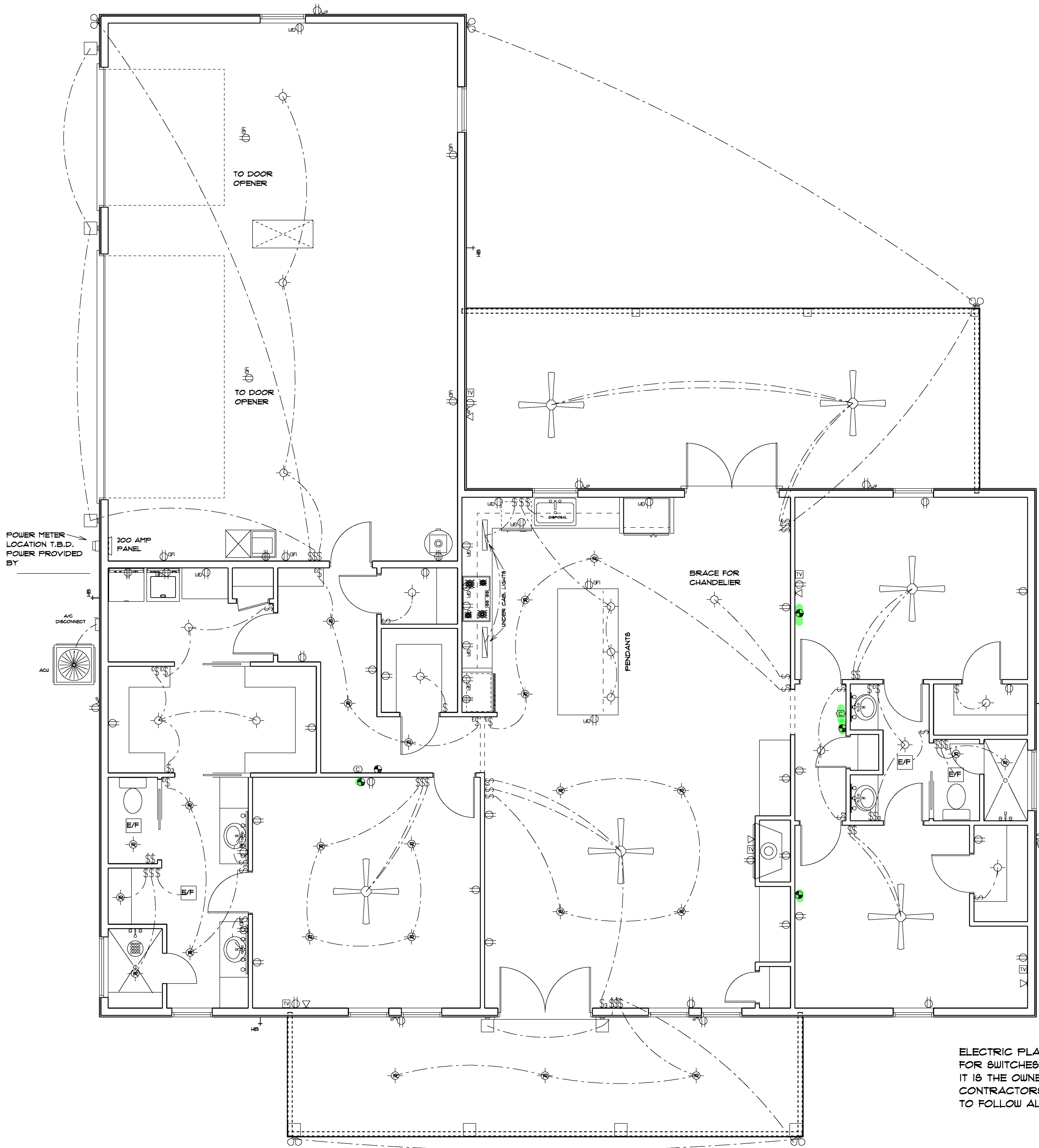
ELECTRICAL PLAN
