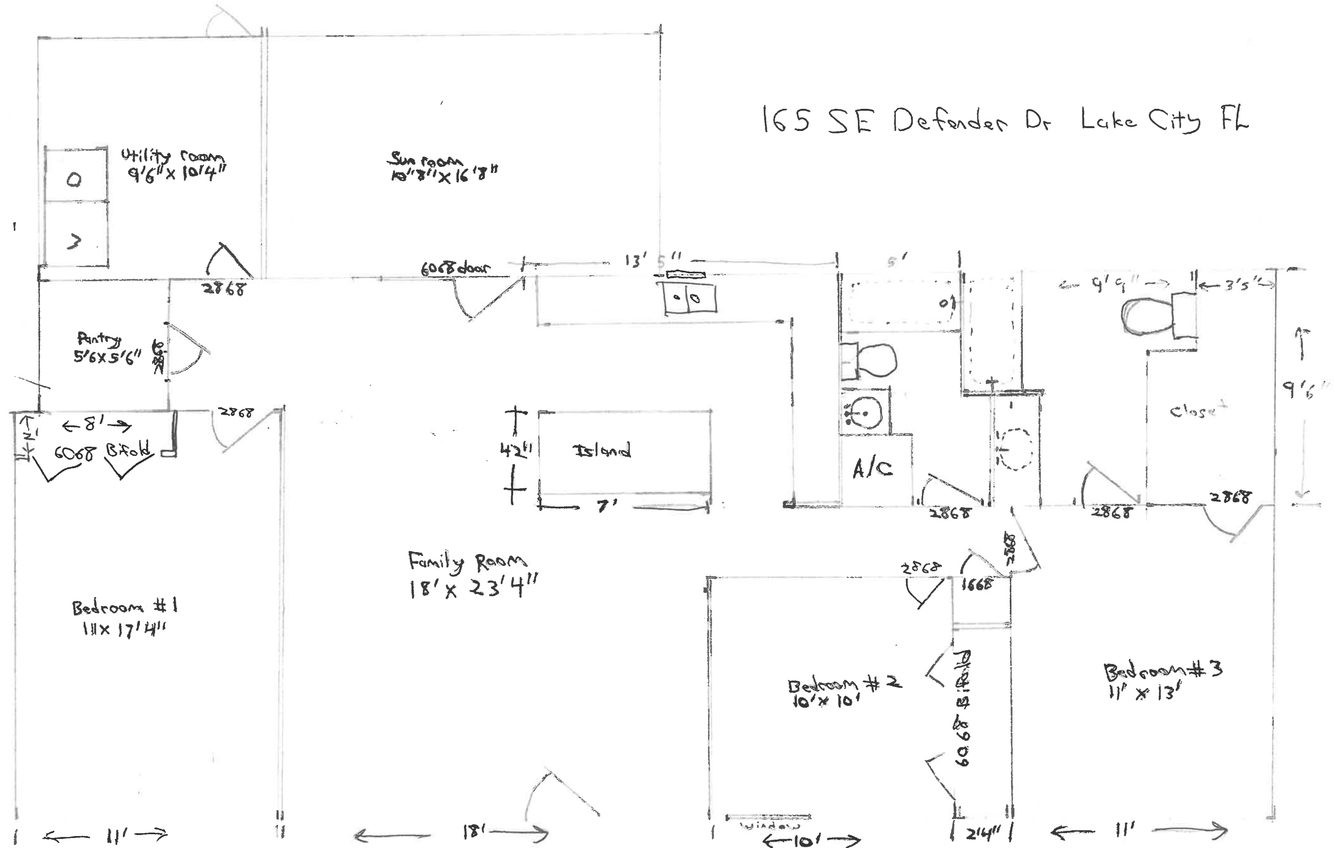
Floor plan
