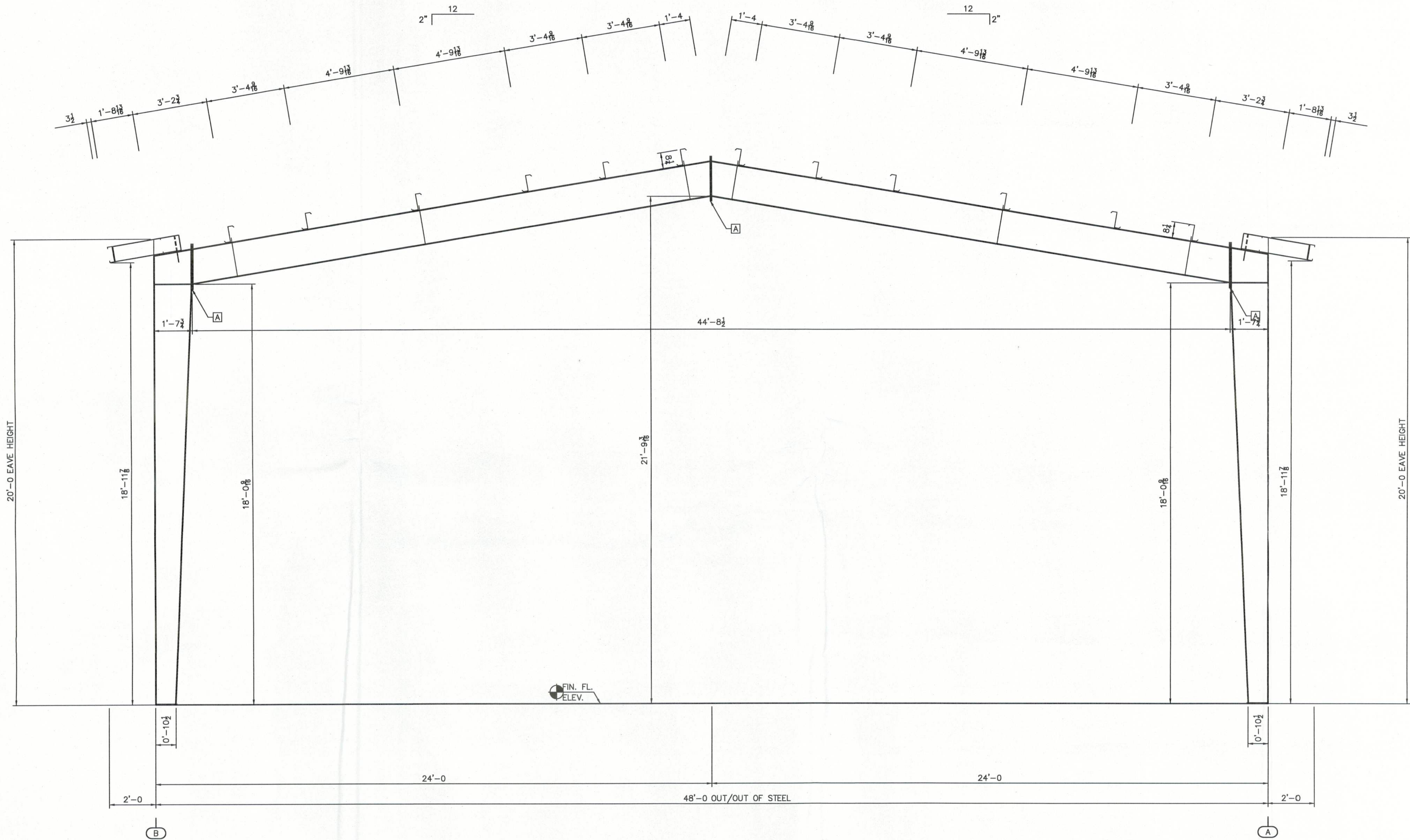
CROSS SECTION AT GRID LINE "4"
