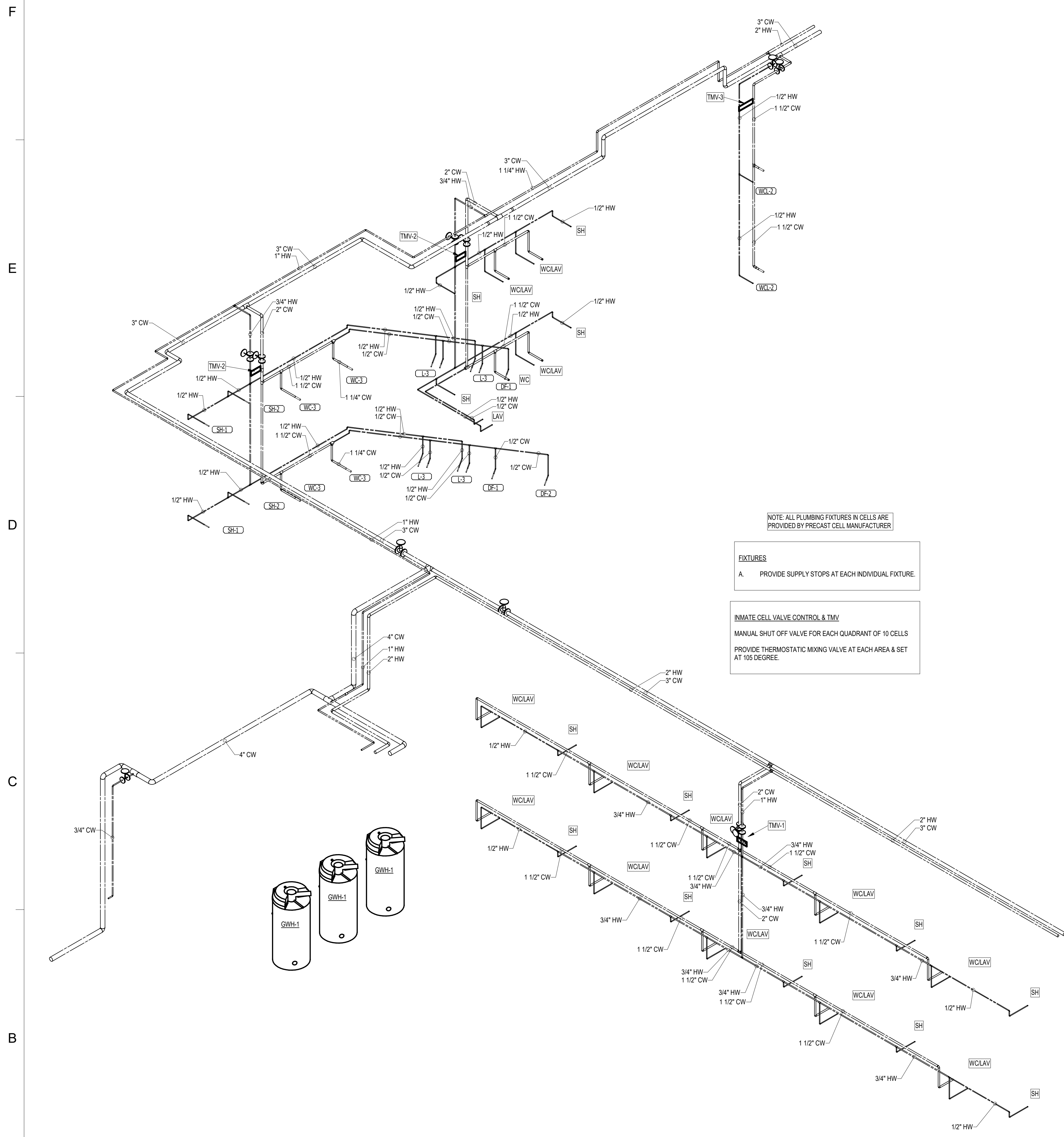
1 PRESSURE RISER-AREA C(SOUTH-SOUTHWEST) Scale:
