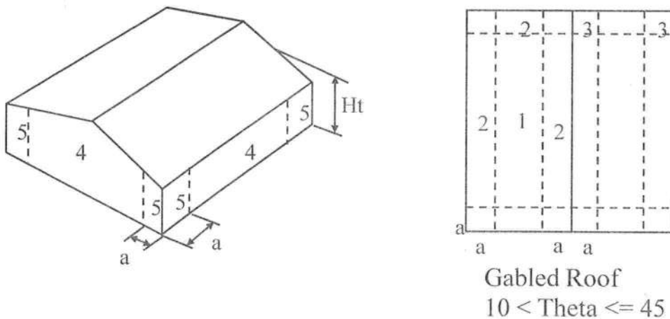
Figure 6-5 - External Pressure Coefficients, GCp Loads on Components and Cladding for Buildings w/ Ht ≤ 60 ft
